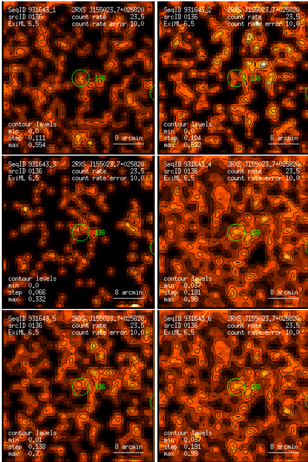
Figure 136: RASS 931643: detection 0136: band rate images, Gaussian filter: (1) PSPC channels 11 – 41, (2) 52 – 90, (3) 91 – 201, (4) 11 – 235, (5) 52 – 201, (6) 11 – 201. Broad band rates in counts/ks. Band rate contour levels in counts/ks/arcmin 2 .
