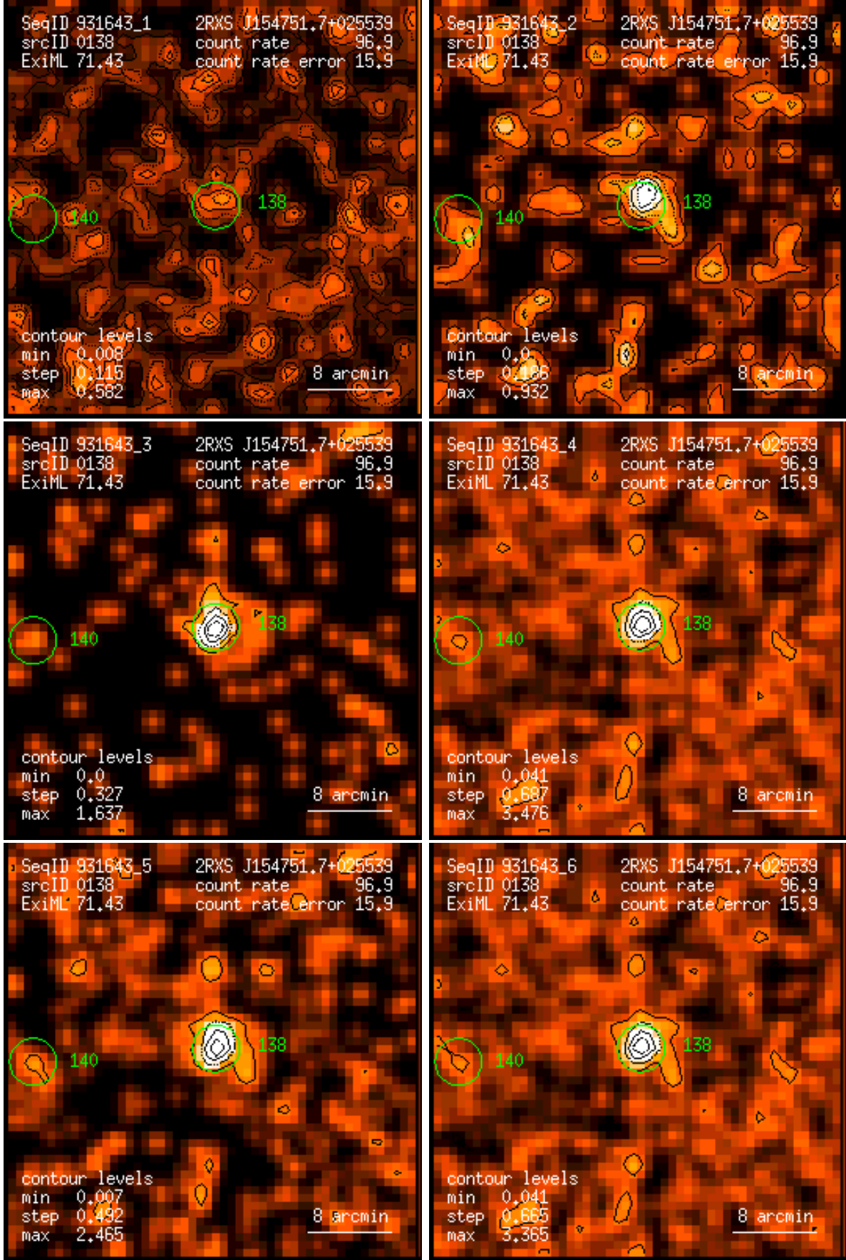
Figure 138: RASS 931643: detection 0138: band rate images, Gaussian filter: (1) PSPC channels 11 – 41, (2) 52 – 90, (3) 91 – 201, (4) 11 – 235, (5) 52 – 201, (6) 11 – 201. Broad band rates in counts/ks. Band rate contour levels in counts/ks/arcmin 2 .
