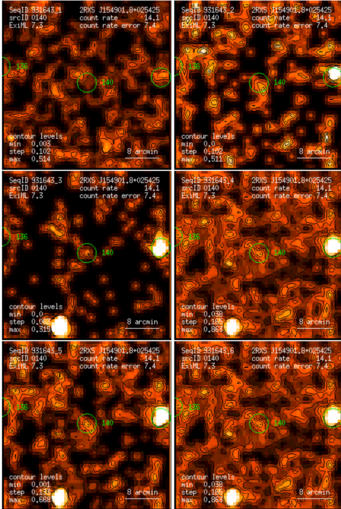
Figure 140: RASS 931643: detection 0140: band rate images, Gaussian filter: (1) PSPC channels 11 – 41, (2) 52 – 90, (3) 91 – 201, (4) 11 – 235, (5) 52 – 201, (6) 11 – 201. Broad band rates in counts/ks. Band rate contour levels in counts/ks/arcmin 2 .
