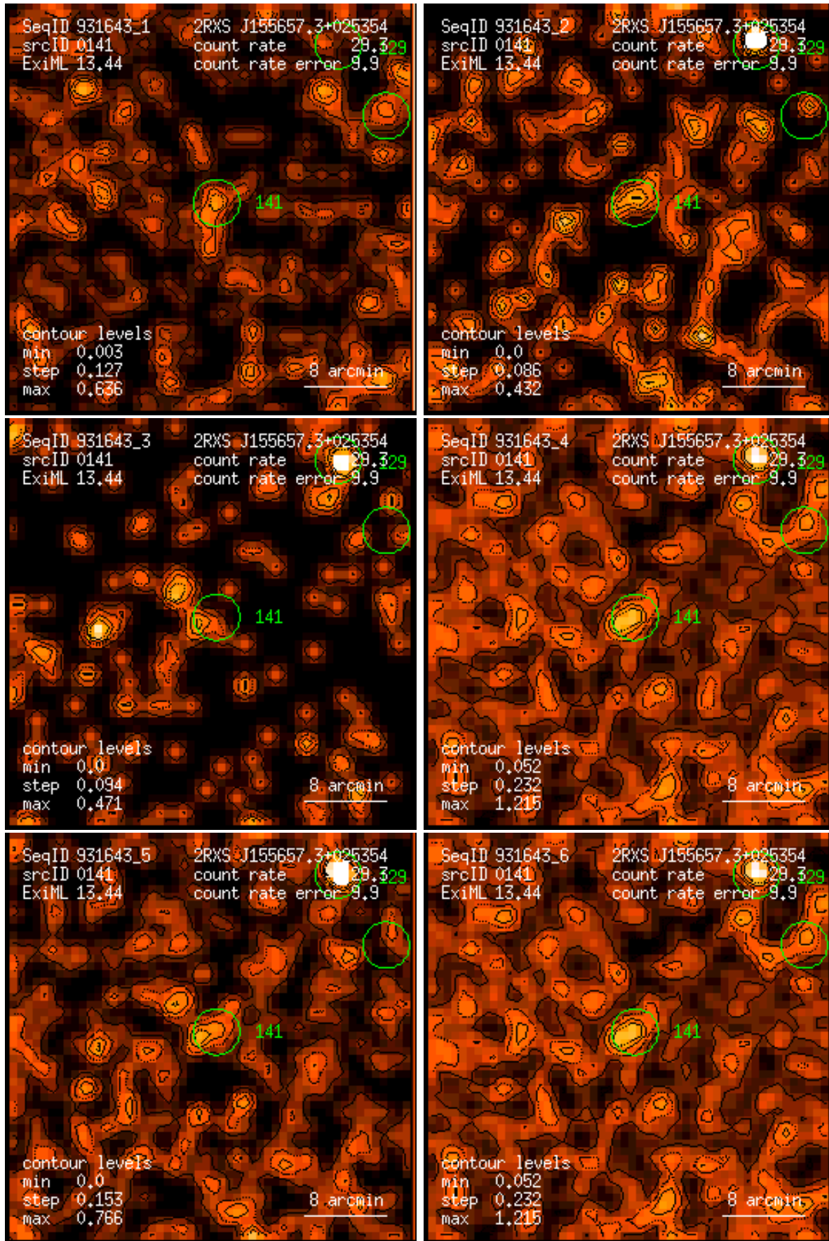
Figure 141: RASS 931643: detection 0141: band rate images, Gaussian filter: (1) PSPC channels 11 – 41, (2) 52 – 90, (3) 91 – 201, (4) 11 – 235, (5) 52 – 201, (6) 11 – 201. Broad band rates in counts/ks. Band rate contour levels in counts/ks/arcmin 2 .
