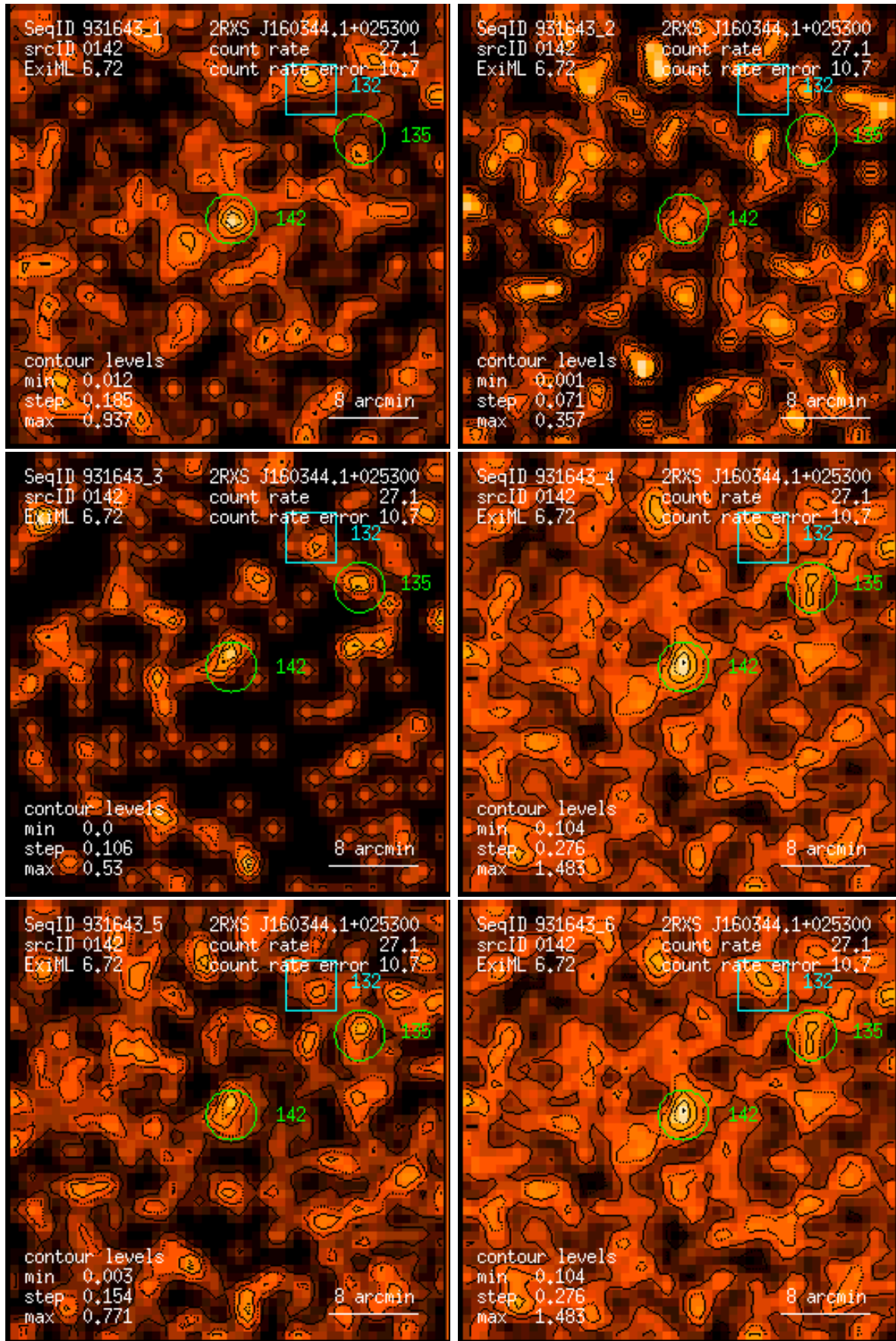
Figure 142: RASS 931643: detection 0142: band rate images, Gaussian filter: (1) PSPC channels 11 – 41, (2) 52 – 90, (3) 91 – 201, (4) 11 – 235, (5) 52 – 201, (6) 11 – 201. Broad band rates in counts/ks. Band rate contour levels in counts/ks/arcmin 2 .
