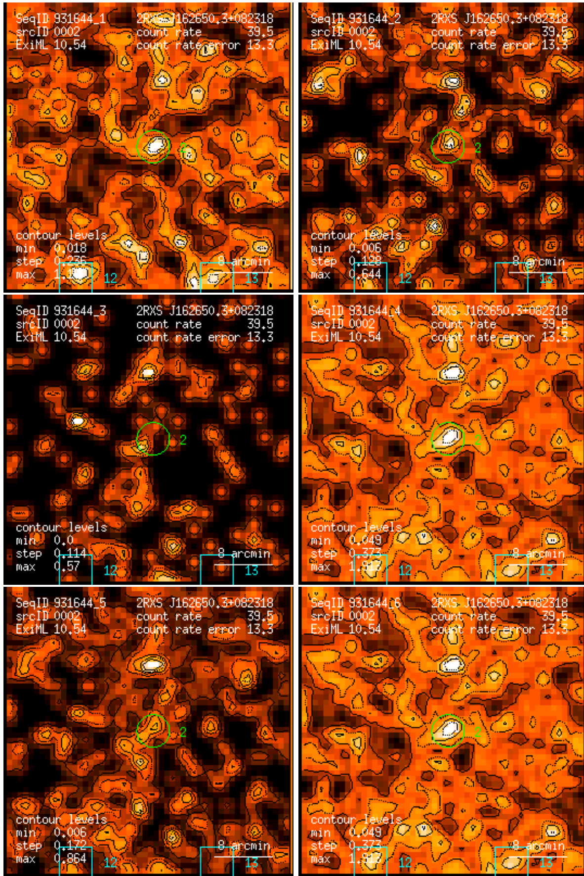
Figure 2: RASS 931644: detection 0002: band rate images, Gaussian filter: (1) PSPC channels 11 – 41, (2) 52 – 90, (3) 91 – 201, (4) 11 – 235, (5) 52 – 201, (6) 11 – 201. Broad band rates in counts/ks. Band rate contour levels in counts/ks/arcmin 2 .
