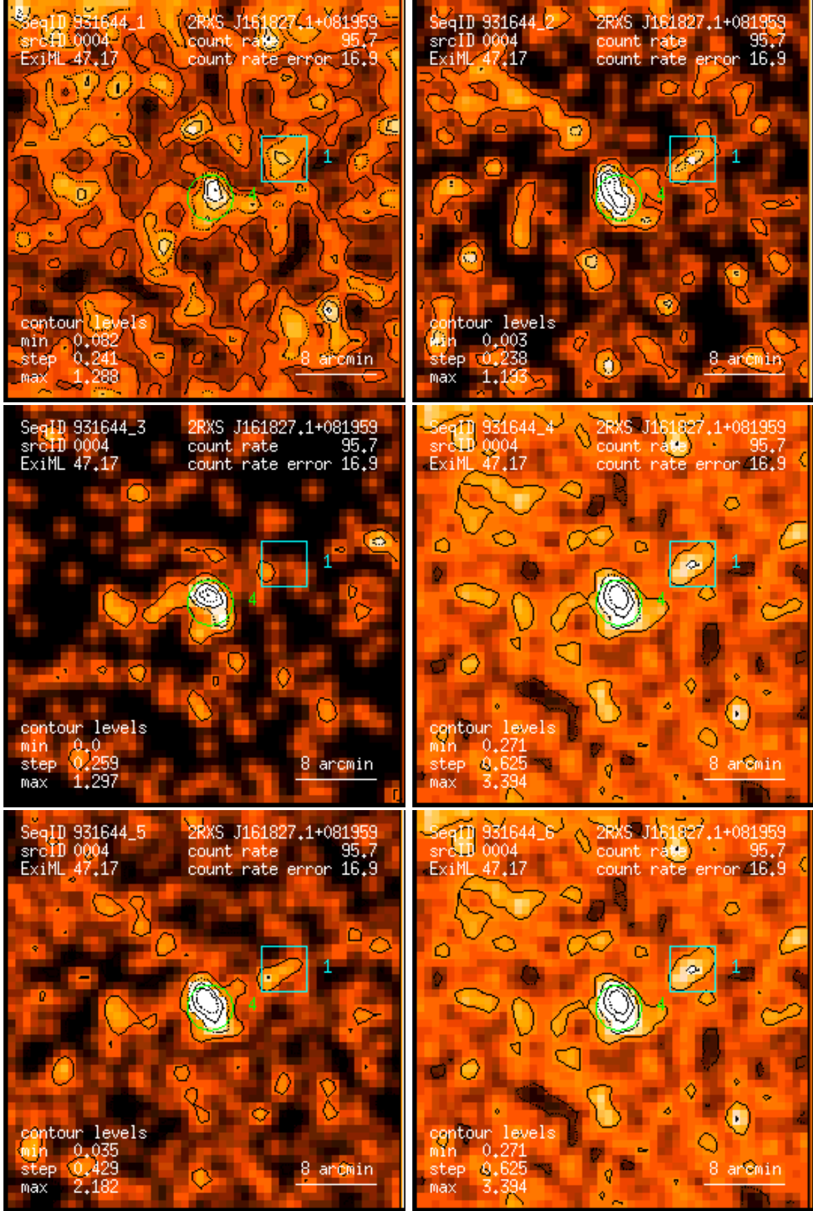
Figure 4: RASS 931644: detection 0004: band rate images, Gaussian filter: (1) PSPC channels 11 – 41, (2) 52 – 90, (3) 91 – 201, (4) 11 – 235, (5) 52 – 201, (6) 11 – 201. Broad band rates in counts/ks. Band rate contour levels in counts/ks/arcmin 2 .
