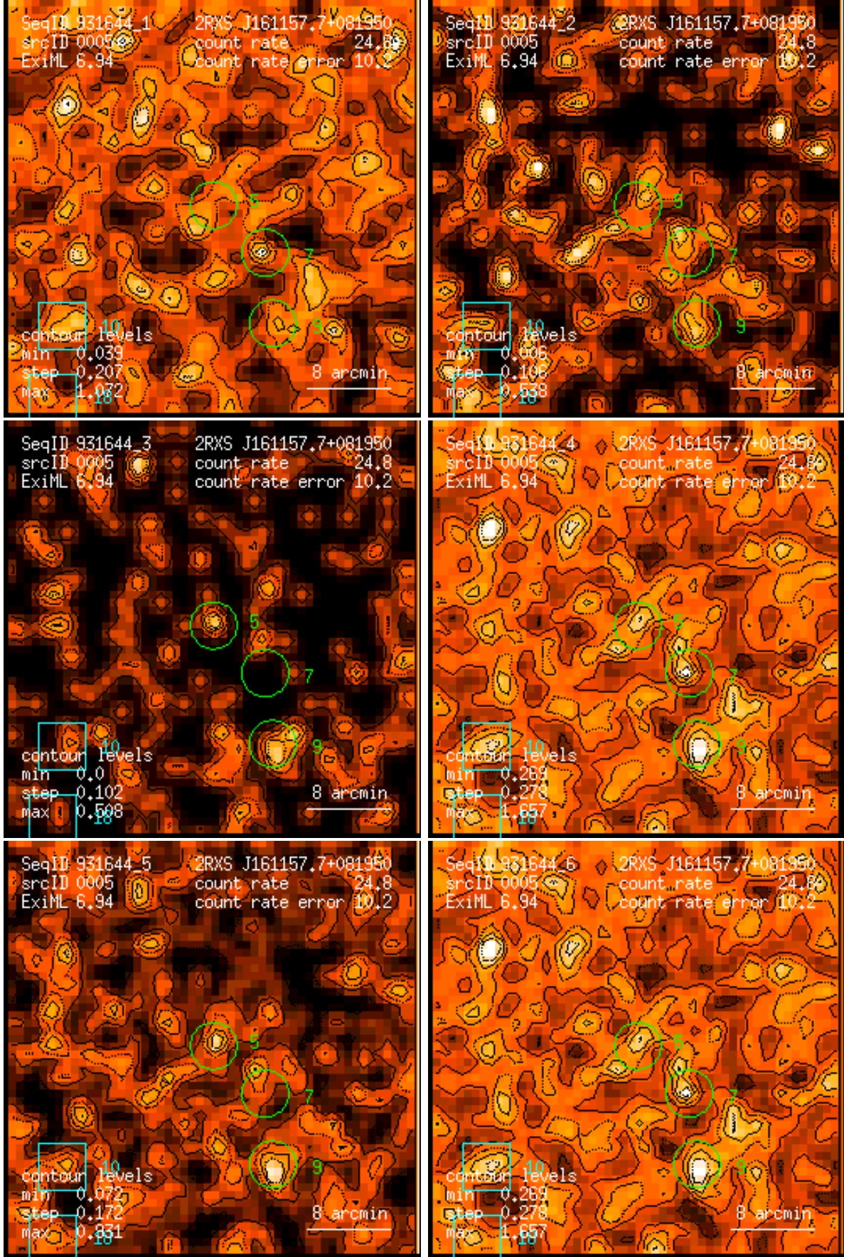
Figure 5: RASS 931644: detection 0005: band rate images, Gaussian filter: (1) PSPC channels 11 – 41, (2) 52 – 90, (3) 91 – 201, (4) 11 – 235, (5) 52 – 201, (6) 11 – 201. Broad band rates in counts/ks. Band rate contour levels in counts/ks/arcmin 2 .
