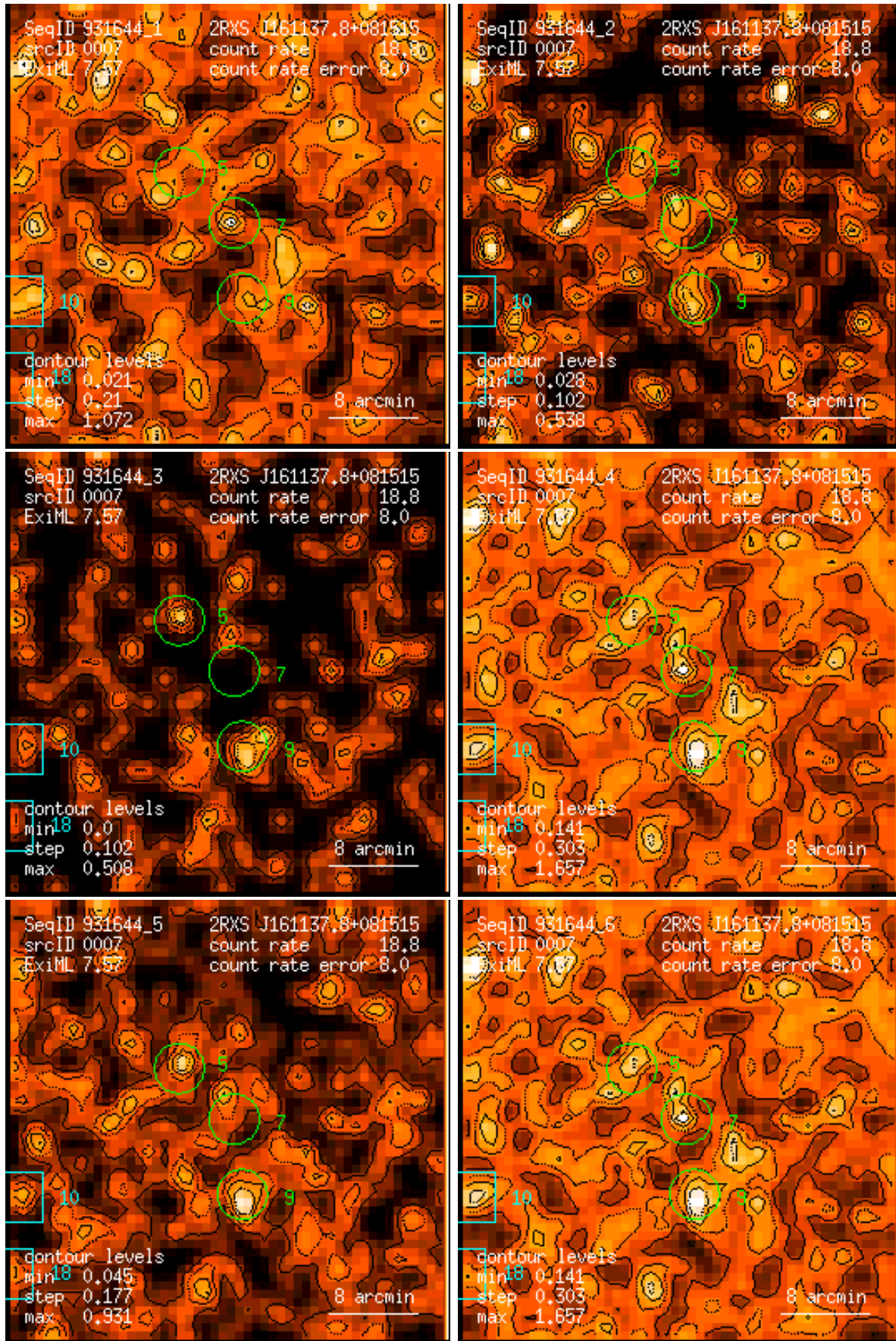
Figure 7: RASS 931644: detection 0007: band rate images, Gaussian filter: (1) PSPC channels 11 – 41, (2) 52 – 90, (3) 91 – 201, (4) 11 – 235, (5) 52 – 201, (6) 11 – 201. Broad band rates in counts/ks. Band rate contour levels in counts/ks/arcmin 2 .
