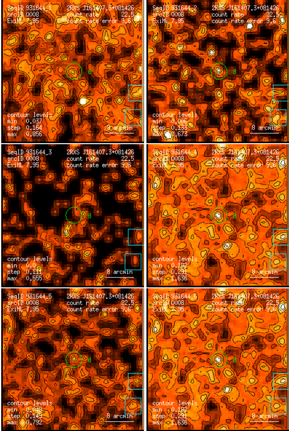
Figure 8: RASS 931644: detection 0008: band rate images, Gaussian filter: (1) PSPC channels 11 – 41, (2) 52 – 90, (3) 91 – 201, (4) 11 – 235, (5) 52 – 201, (6) 11 – 201. Broad band rates in counts/ks. Band rate contour levels in counts/ks/arcmin 2 .
