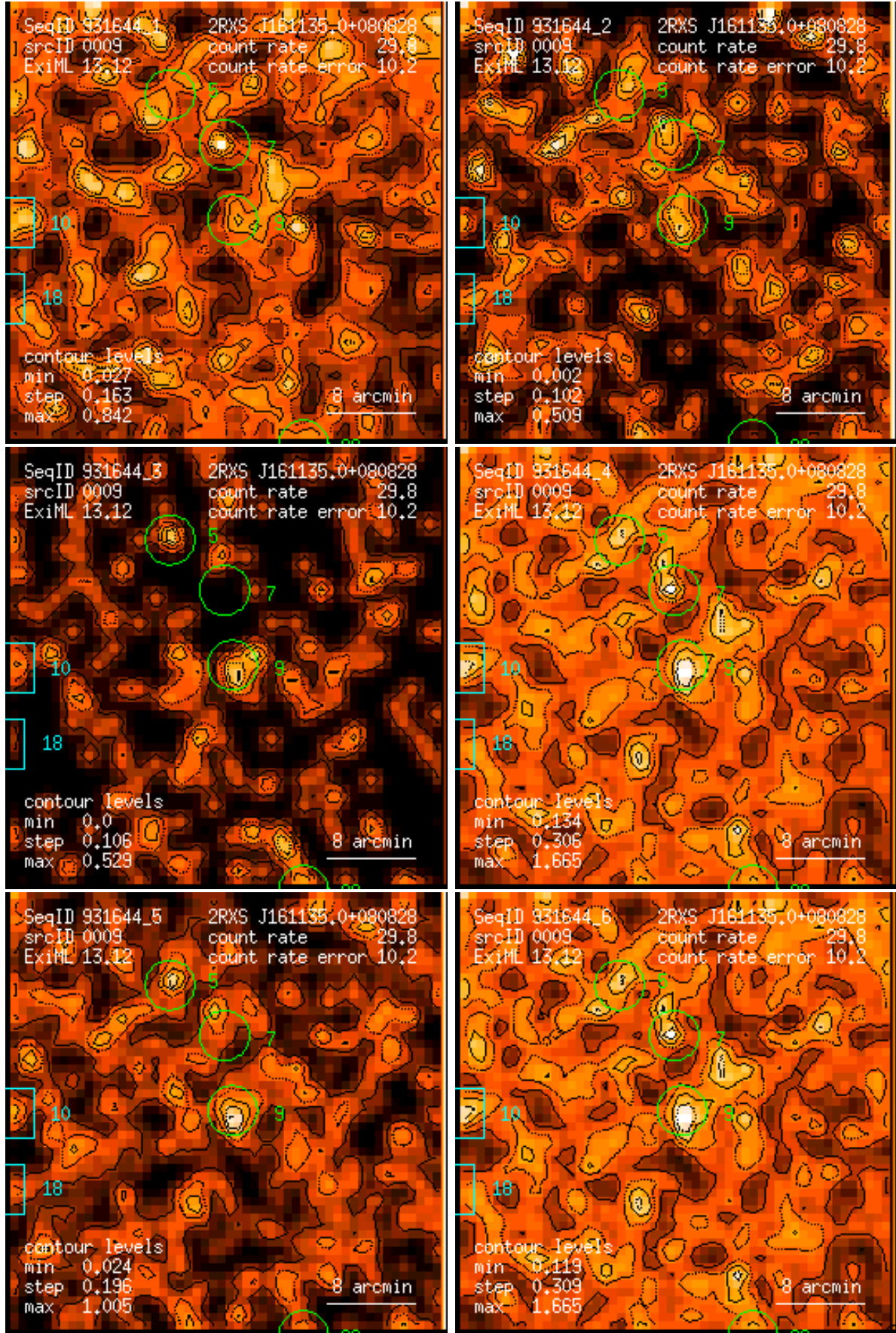
Figure 9: RASS 931644: detection 0009: band rate images, Gaussian filter: (1) PSPC channels 11 – 41, (2) 52 – 90, (3) 91 – 201, (4) 11 – 235, (5) 52 – 201, (6) 11 – 201. Broad band rates in counts/ks. Band rate contour levels in counts/ks/arcmin 2 .
