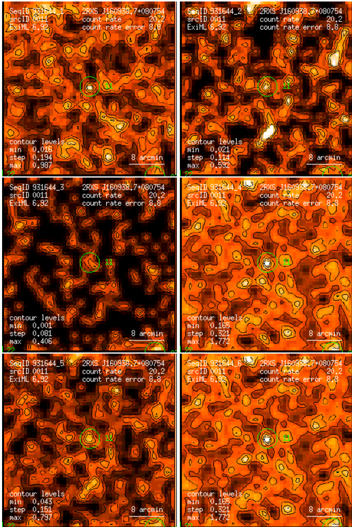
Figure 11: RASS 931644: detection 0011: band rate images, Gaussian filter: (1) PSPC channels 11 – 41, (2) 52 – 90, (3) 91 – 201, (4) 11 – 235, (5) 52 – 201, (6) 11 – 201. Broad band rates in counts/ks. Band rate contour levels in counts/ks/arcmin 2 .
