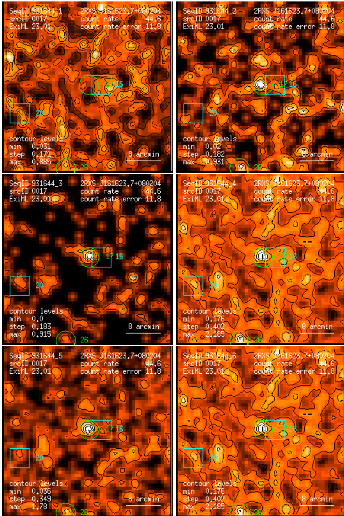
Figure 17: RASS 931644: detection 0017: band rate images, Gaussian filter: (1) PSPC channels 11 – 41, (2) 52 – 90, (3) 91 – 201, (4) 11 – 235, (5) 52 – 201, (6) 11 – 201. Broad band rates in counts/ks. Band rate contour levels in counts/ks/arcmin 2 .
