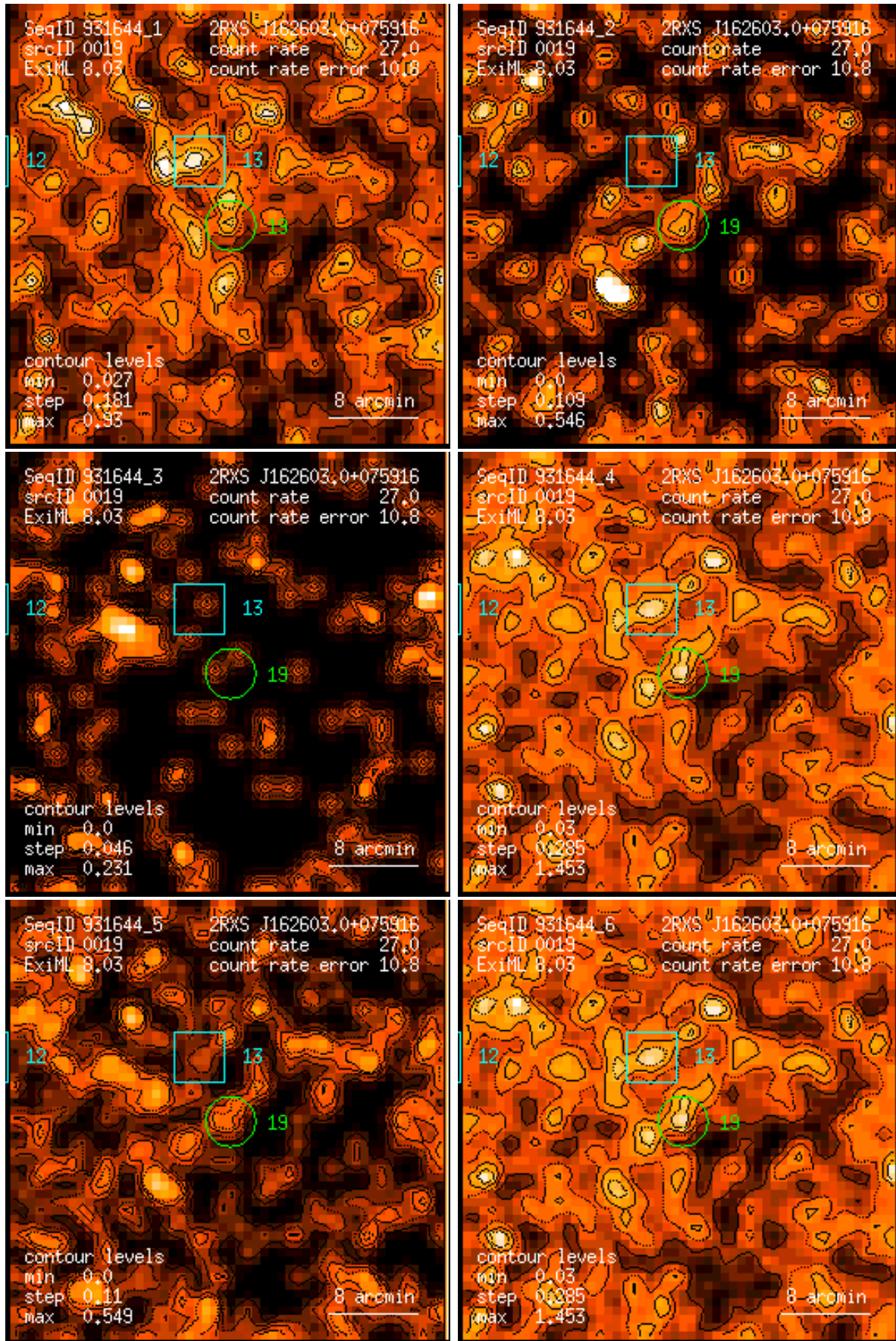
Figure 19: RASS 931644: detection 0019: band rate images, Gaussian filter: (1) PSPC channels 11 – 41, (2) 52 – 90, (3) 91 – 201, (4) 11 – 235, (5) 52 – 201, (6) 11 – 201. Broad band rates in counts/ks. Band rate contour levels in counts/ks/arcmin 2 .
