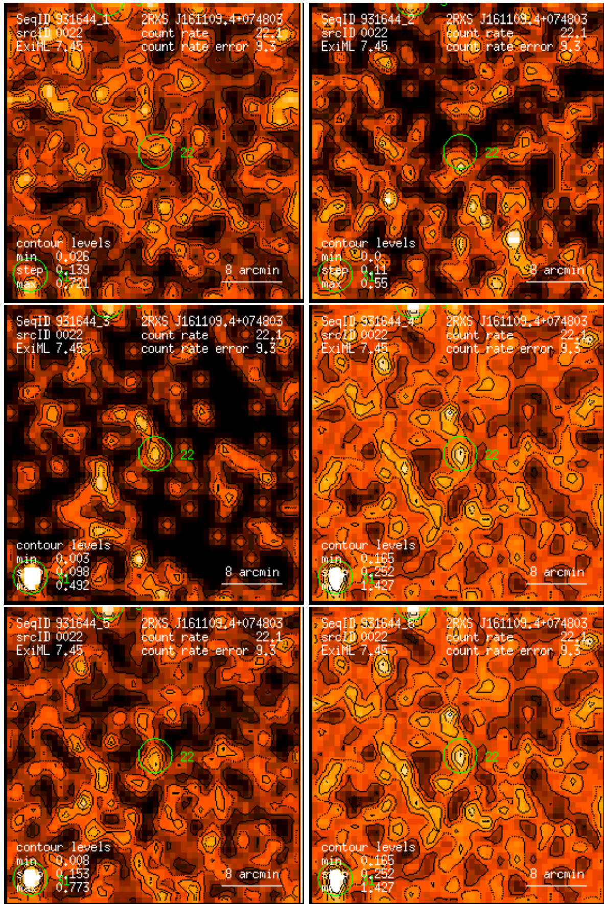
Figure 22: RASS 931644: detection 0022: band rate images, Gaussian filter: (1) PSPC channels 11 – 41, (2) 52 – 90, (3) 91 – 201, (4) 11 – 235, (5) 52 – 201, (6) 11 – 201. Broad band rates in counts/ks. Band rate contour levels in counts/ks/arcmin 2 .
