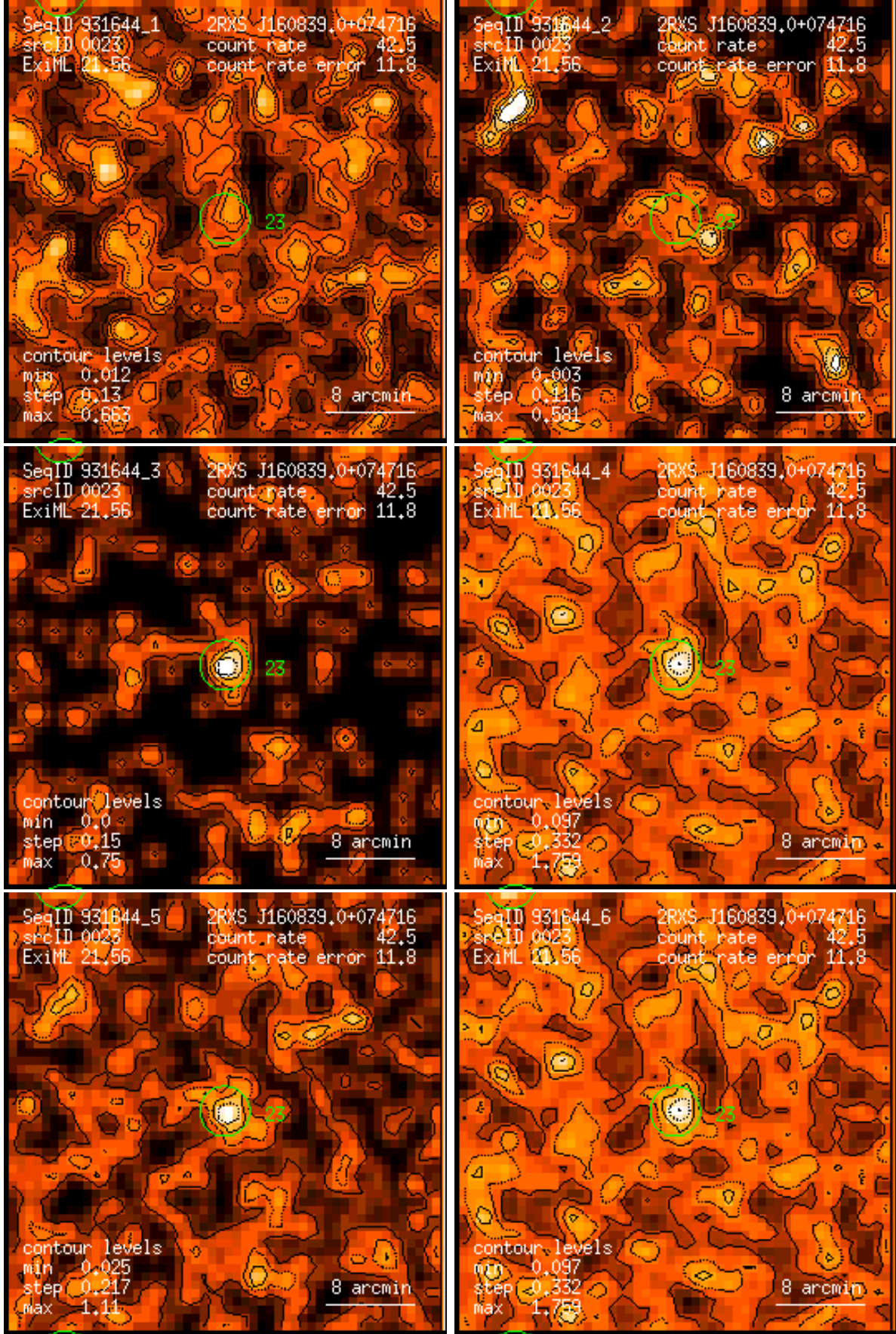
Figure 23: RASS 931644: detection 0023: band rate images, Gaussian filter: (1) PSPC channels 11 – 41, (2) 52 – 90, (3) 91 – 201, (4) 11 – 235, (5) 52 – 201, (6) 11 – 201. Broad band rates in counts/ks. Band rate contour levels in counts/ks/arcmin 2 .
