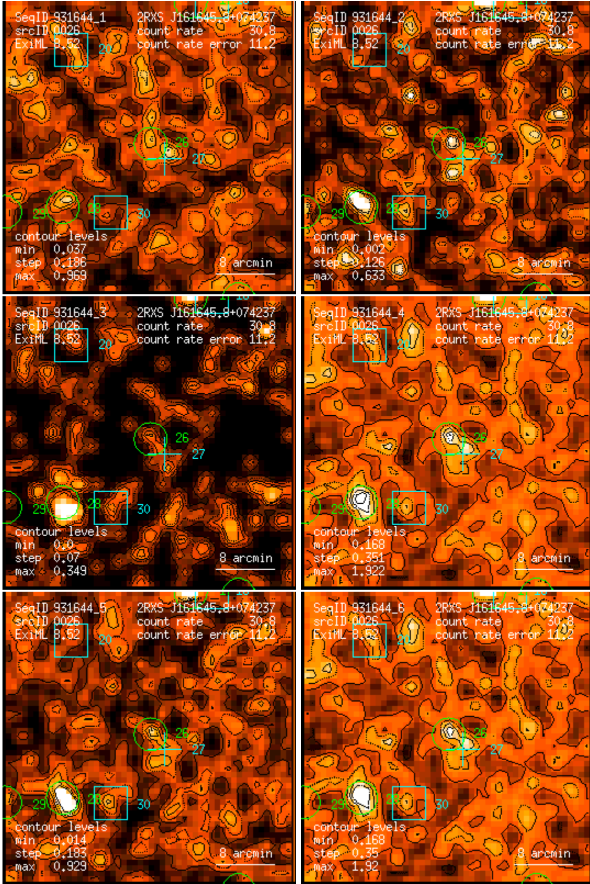
Figure 26: RASS 931644: detection 0026: band rate images, Gaussian filter: (1) PSPC channels 11 – 41, (2) 52 – 90, (3) 91 – 201, (4) 11 – 235, (5) 52 – 201, (6) 11 – 201. Broad band rates in counts/ks. Band rate contour levels in counts/ks/arcmin 2 .
