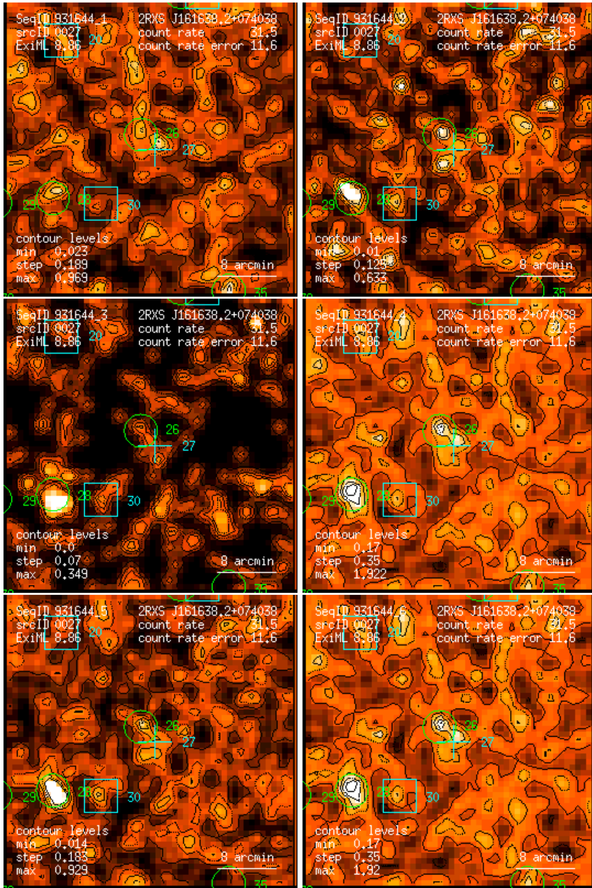
Figure 27: RASS 931644: detection 0027: band rate images, Gaussian filter: (1) PSPC channels 11 – 41, (2) 52 – 90, (3) 91 – 201, (4) 11 – 235, (5) 52 – 201, (6) 11 – 201. Broad band rates in counts/ks. Band rate contour levels in counts/ks/arcmin 2 .
