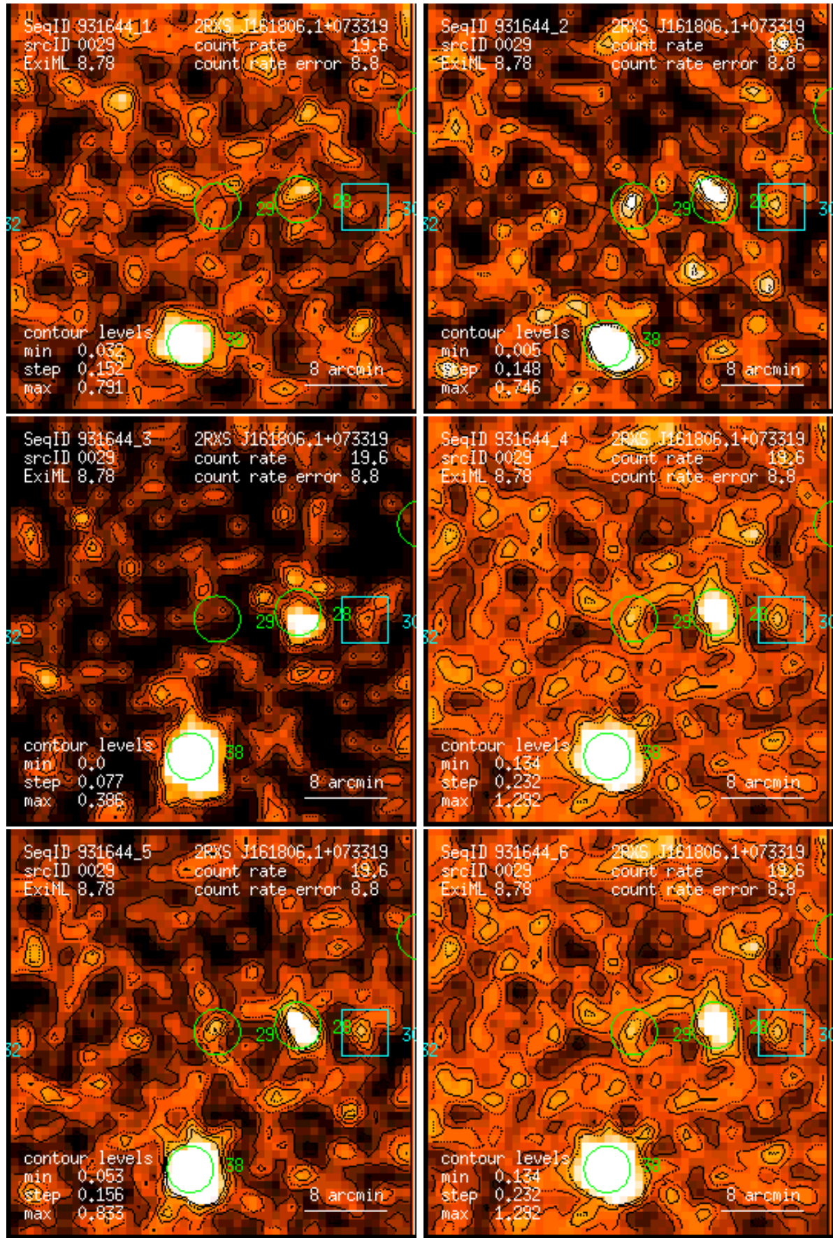
Figure 29: RASS 931644: detection 0029: band rate images, Gaussian filter: (1) PSPC channels 11 – 41, (2) 52 – 90, (3) 91 – 201, (4) 11 – 235, (5) 52 – 201, (6) 11 – 201. Broad band rates in counts/ks. Band rate contour levels in counts/ks/arcmin 2 .
