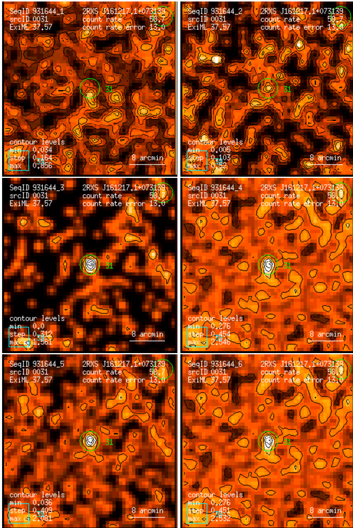
Figure 31: RASS 931644: detection 0031: band rate images, Gaussian filter: (1) PSPC channels 11 – 41, (2) 52 – 90, (3) 91 – 201, (4) 11 – 235, (5) 52 – 201, (6) 11 – 201. Broad band rates in counts/ks. Band rate contour levels in counts/ks/arcmin 2 .
