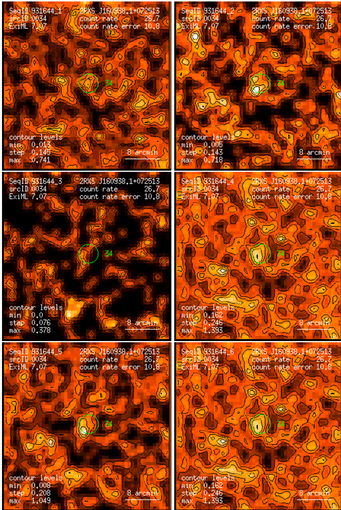
Figure 34: RASS 931644: detection 0034: band rate images, Gaussian filter: (1) PSPC channels 11 – 41, (2) 52 – 90, (3) 91 – 201, (4) 11 – 235, (5) 52 – 201, (6) 11 – 201. Broad band rates in counts/ks. Band rate contour levels in counts/ks/arcmin 2 .
