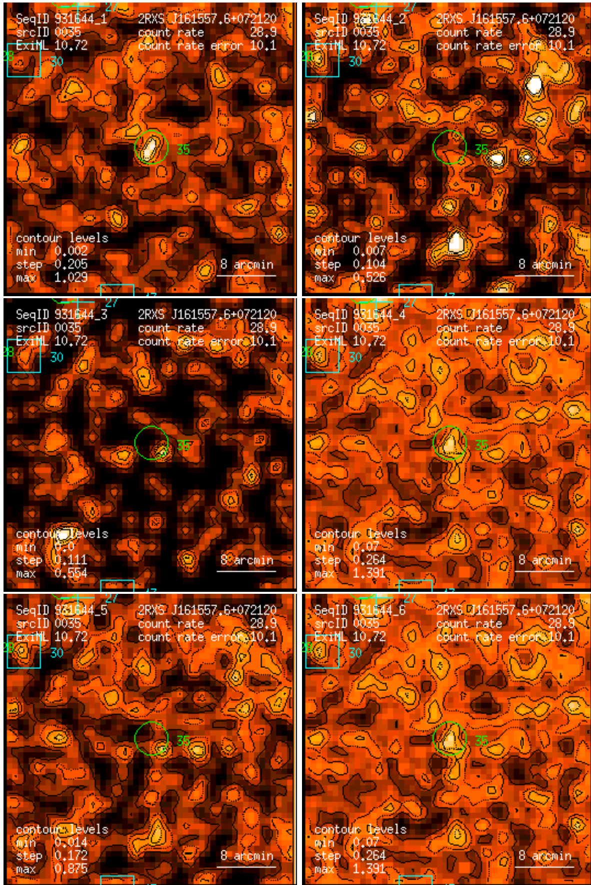
Figure 35: RASS 931644: detection 0035: band rate images, Gaussian filter: (1) PSPC channels 11 – 41, (2) 52 – 90, (3) 91 – 201, (4) 11 – 235, (5) 52 – 201, (6) 11 – 201. Broad band rates in counts/ks. Band rate contour levels in counts/ks/arcmin 2 .
