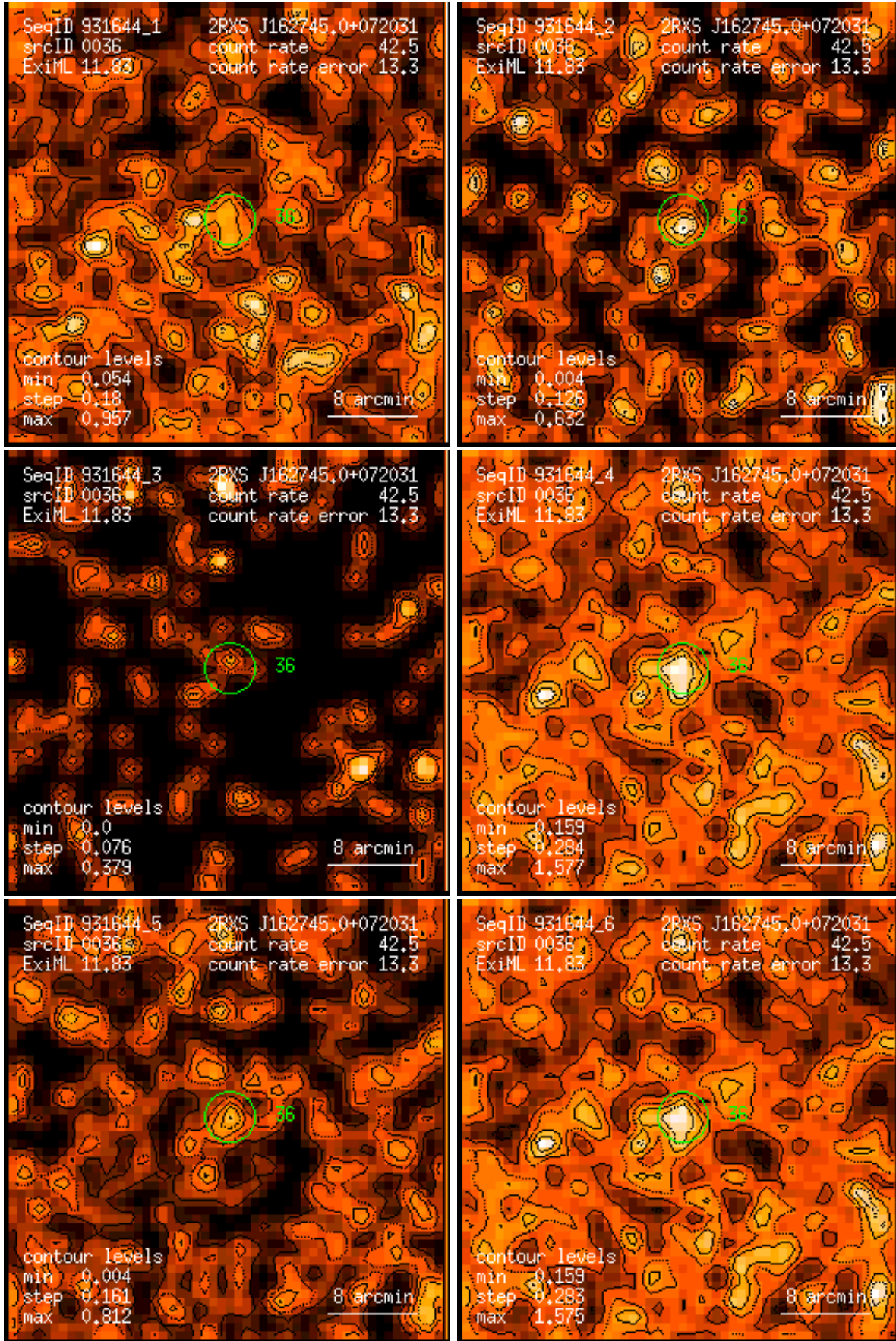
Figure 36: RASS 931644: detection 0036: band rate images, Gaussian filter: (1) PSPC channels 11 – 41, (2) 52 – 90, (3) 91 – 201, (4) 11 – 235, (5) 52 – 201, (6) 11 – 201. Broad band rates in counts/ks. Band rate contour levels in counts/ks/arcmin 2 .
