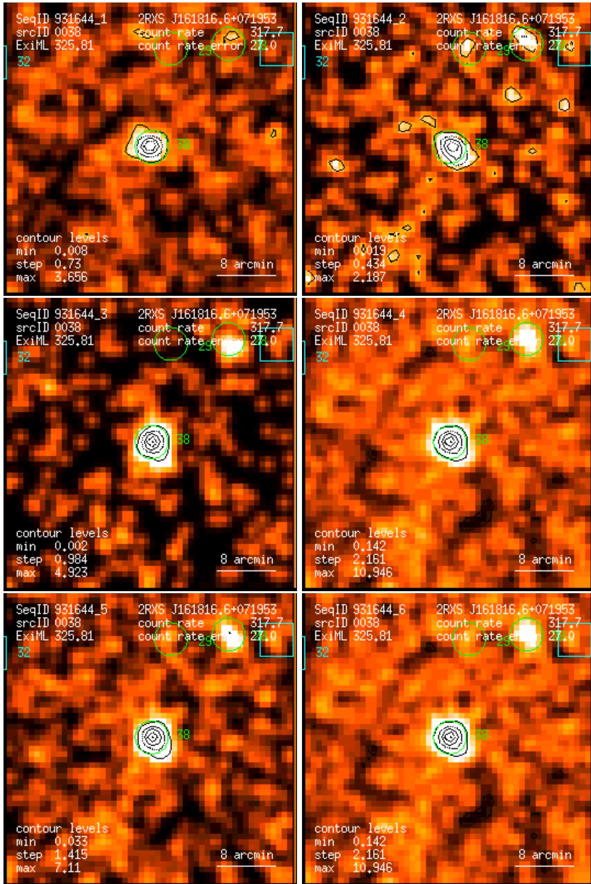
Figure 38: RASS 931644: detection 0038: band rate images, Gaussian filter: (1) PSPC channels 11 – 41, (2) 52 – 90, (3) 91 – 201, (4) 11 – 235, (5) 52 – 201, (6) 11 – 201. Broad band rates in counts/ks. Band rate contour levels in counts/ks/arcmin 2 .
