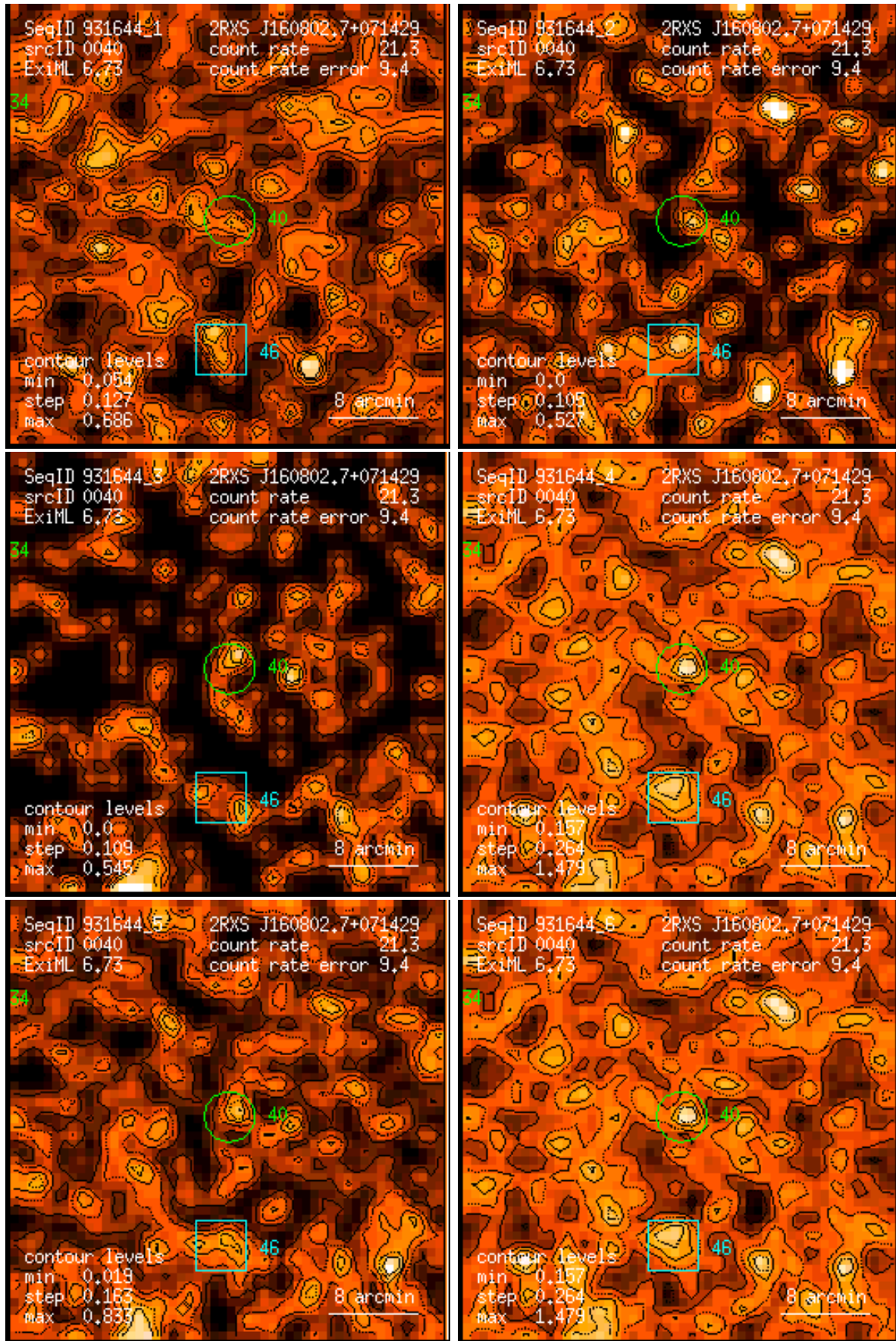
Figure 40: RASS 931644: detection 0040: band rate images, Gaussian filter: (1) PSPC channels 11 – 41, (2) 52 – 90, (3) 91 – 201, (4) 11 – 235, (5) 52 – 201, (6) 11 – 201. Broad band rates in counts/ks. Band rate contour levels in counts/ks/arcmin 2 .
