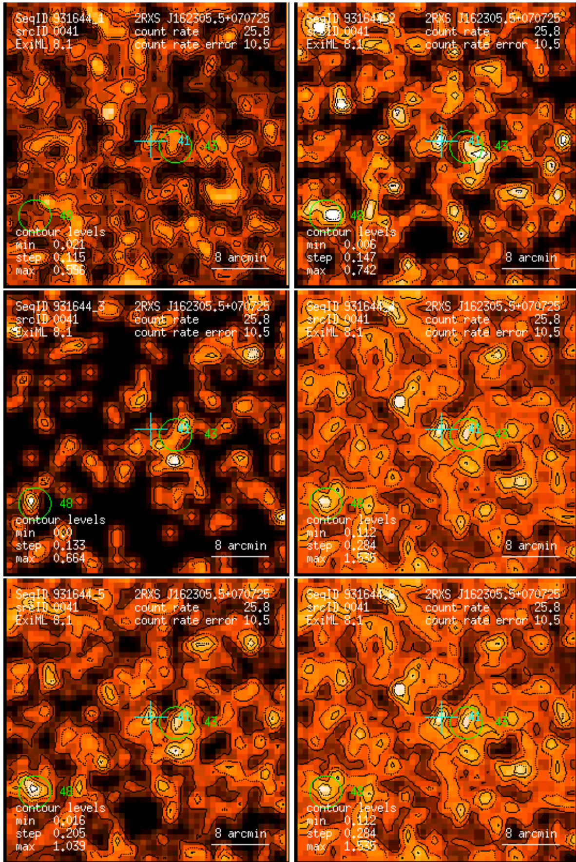
Figure 41: RASS 931644: detection 0041: band rate images, Gaussian filter: (1) PSPC channels 11 – 41, (2) 52 – 90, (3) 91 – 201, (4) 11 – 235, (5) 52 – 201, (6) 11 – 201. Broad band rates in counts/ks. Band rate contour levels in counts/ks/arcmin 2 .
