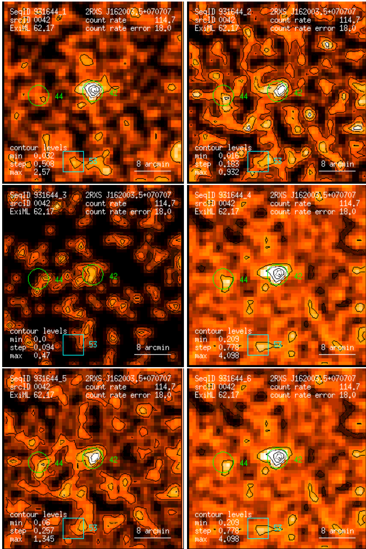
Figure 42: RASS 931644: detection 0042: band rate images, Gaussian filter: (1) PSPC channels 11 – 41, (2) 52 – 90, (3) 91 – 201, (4) 11 – 235, (5) 52 – 201, (6) 11 – 201. Broad band rates in counts/ks. Band rate contour levels in counts/ks/arcmin 2 .
