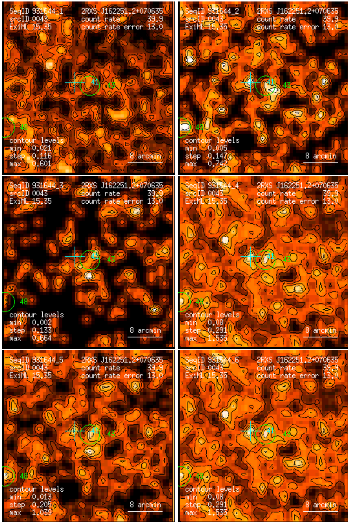
Figure 43: RASS 931644: detection 0043: band rate images, Gaussian filter: (1) PSPC channels 11 – 41, (2) 52 – 90, (3) 91 – 201, (4) 11 – 235, (5) 52 – 201, (6) 11 – 201. Broad band rates in counts/ks. Band rate contour levels in counts/ks/arcmin 2 .
