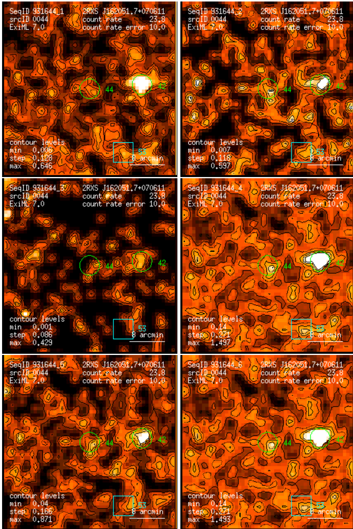
Figure 44: RASS 931644: detection 0044: band rate images, Gaussian filter: (1) PSPC channels 11 – 41, (2) 52 – 90, (3) 91 – 201, (4) 11 – 235, (5) 52 – 201, (6) 11 – 201. Broad band rates in counts/ks. Band rate contour levels in counts/ks/arcmin 2 .
