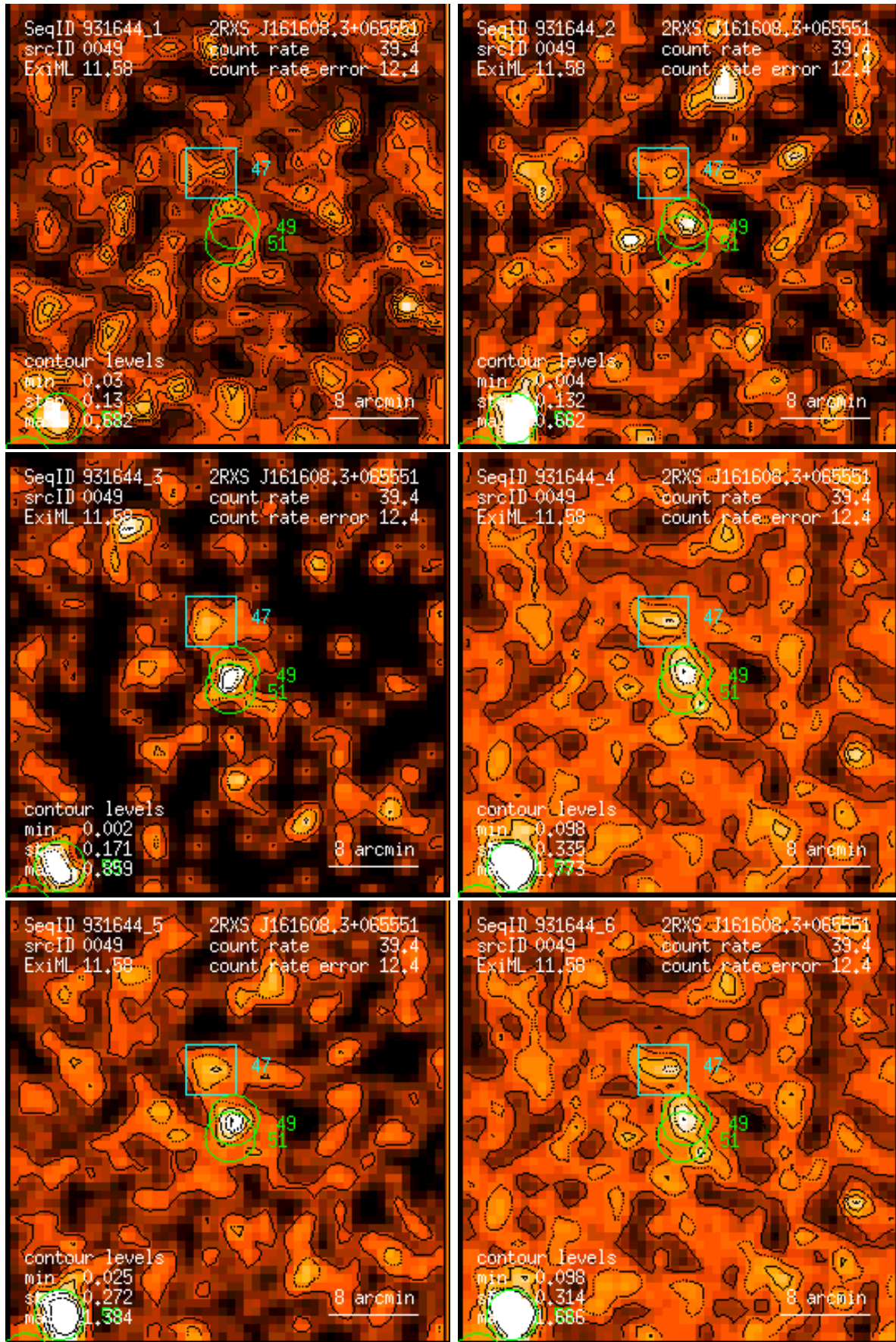
Figure 49: RASS 931644: detection 0049: band rate images, Gaussian filter: (1) PSPC channels 11 – 41, (2) 52 – 90, (3) 91 – 201, (4) 11 – 235, (5) 52 – 201, (6) 11 – 201. Broad band rates in counts/ks. Band rate contour levels in counts/ks/arcmin 2 .
