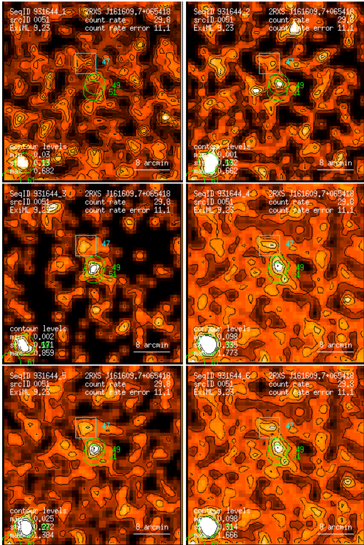
Figure 51: RASS 931644: detection 0051: band rate images, Gaussian filter: (1) PSPC channels 11 – 41, (2) 52 – 90, (3) 91 – 201, (4) 11 – 235, (5) 52 – 201, (6) 11 – 201. Broad band rates in counts/ks. Band rate contour levels in counts/ks/arcmin 2 .
