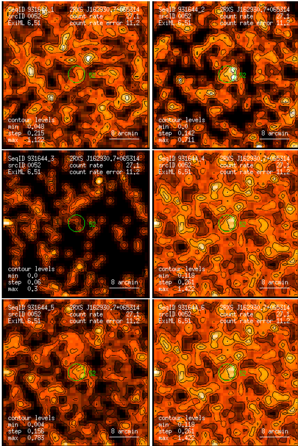
Figure 52: RASS 931644: detection 0052: band rate images, Gaussian filter: (1) PSPC channels 11 – 41, (2) 52 – 90, (3) 91 – 201, (4) 11 – 235, (5) 52 – 201, (6) 11 – 201. Broad band rates in counts/ks. Band rate contour levels in counts/ks/arcmin 2 .
