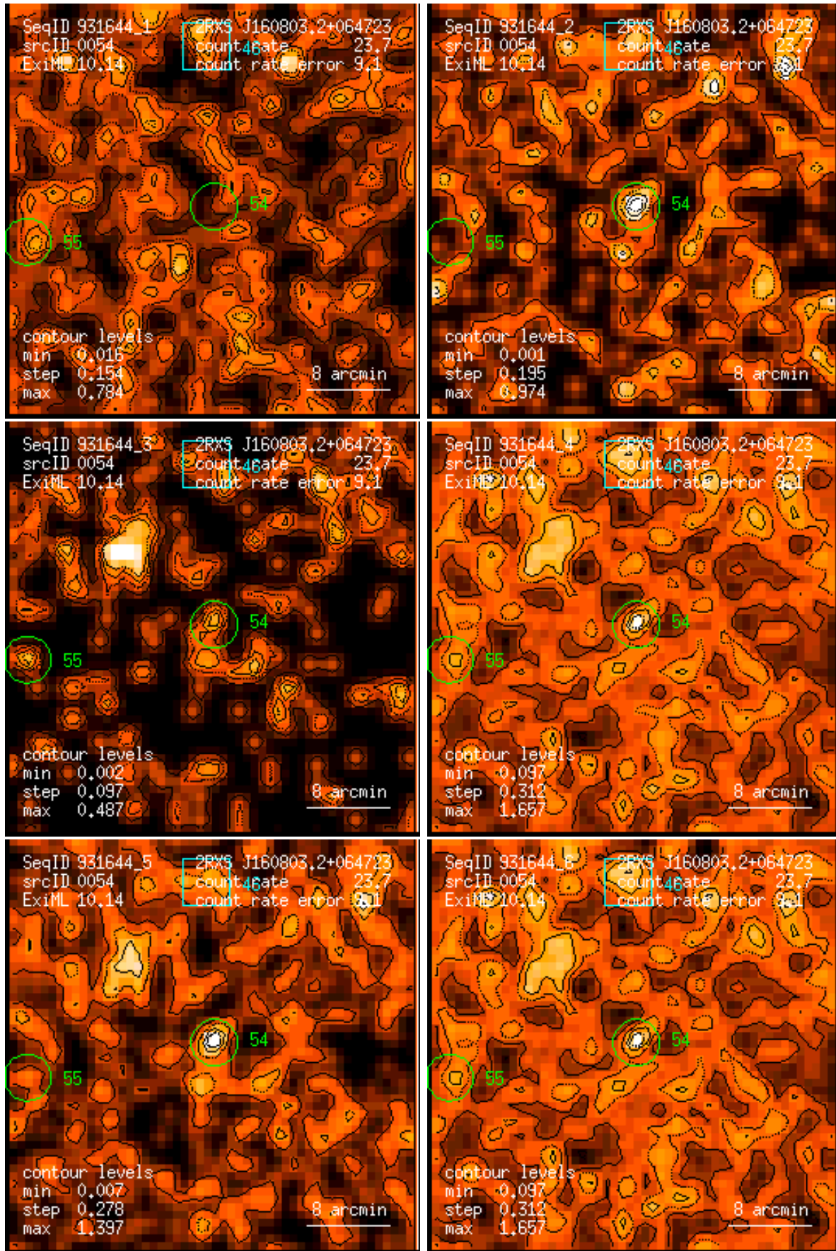
Figure 54: RASS 931644: detection 0054: band rate images, Gaussian filter: (1) PSPC channels 11 – 41, (2) 52 – 90, (3) 91 – 201, (4) 11 – 235, (5) 52 – 201, (6) 11 – 201. Broad band rates in counts/ks. Band rate contour levels in counts/ks/arcmin 2 .
