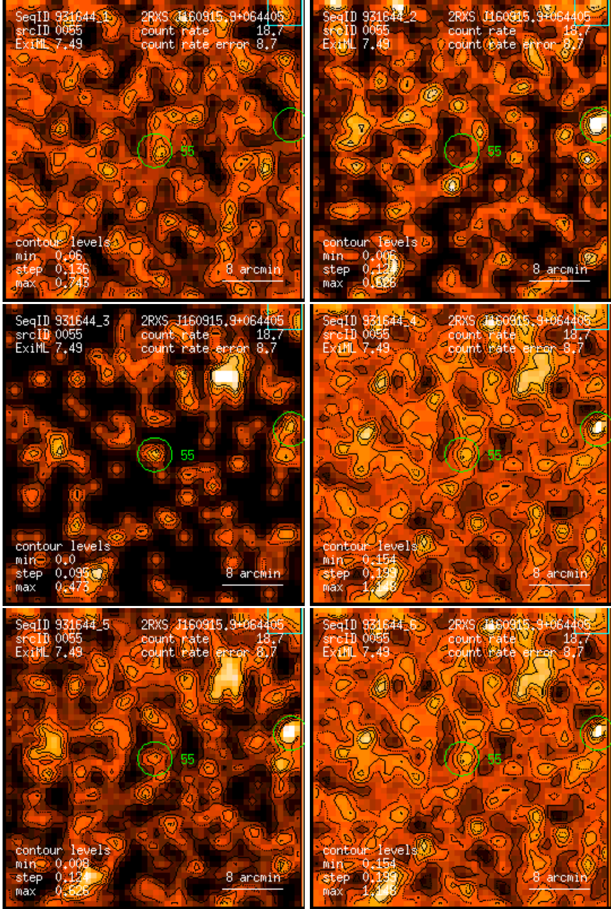
Figure 55: RASS 931644: detection 0055: band rate images, Gaussian filter: (1) PSPC channels 11 – 41, (2) 52 – 90, (3) 91 – 201, (4) 11 – 235, (5) 52 – 201, (6) 11 – 201. Broad band rates in counts/ks. Band rate contour levels in counts/ks/arcmin 2 .
