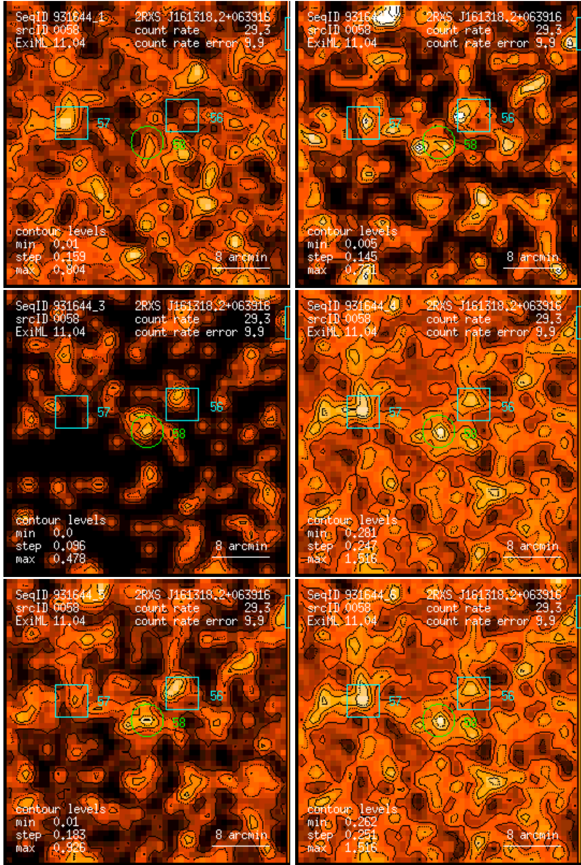
Figure 58: RASS 931644: detection 0058: band rate images, Gaussian filter: (1) PSPC channels 11 – 41, (2) 52 – 90, (3) 91 – 201, (4) 11 – 235, (5) 52 – 201, (6) 11 – 201. Broad band rates in counts/ks. Band rate contour levels in counts/ks/arcmin 2 .
