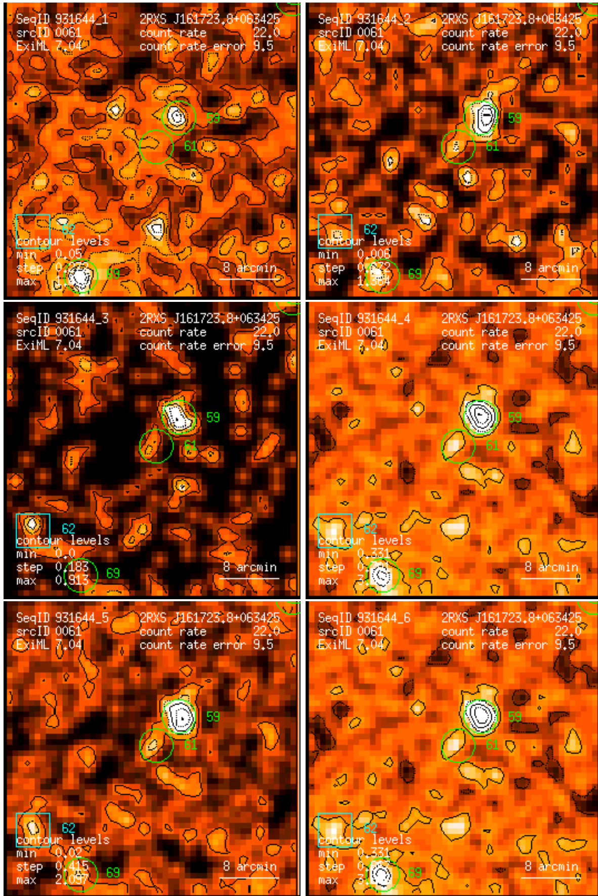
Figure 61: RASS 931644: detection 0061: band rate images, Gaussian filter: (1) PSPC channels 11 – 41, (2) 52 – 90, (3) 91 – 201, (4) 11 – 235, (5) 52 – 201, (6) 11 – 201. Broad band rates in counts/ks. Band rate contour levels in counts/ks/arcmin 2 .
