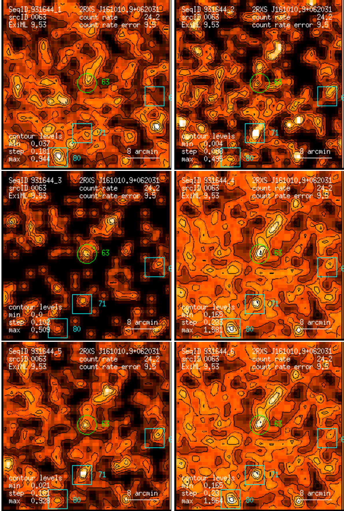
Figure 63: RASS 931644: detection 0063: band rate images, Gaussian filter: (1) PSPC channels 11 – 41, (2) 52 – 90, (3) 91 – 201, (4) 11 – 235, (5) 52 – 201, (6) 11 – 201. Broad band rates in counts/ks. Band rate contour levels in counts/ks/arcmin 2 .
