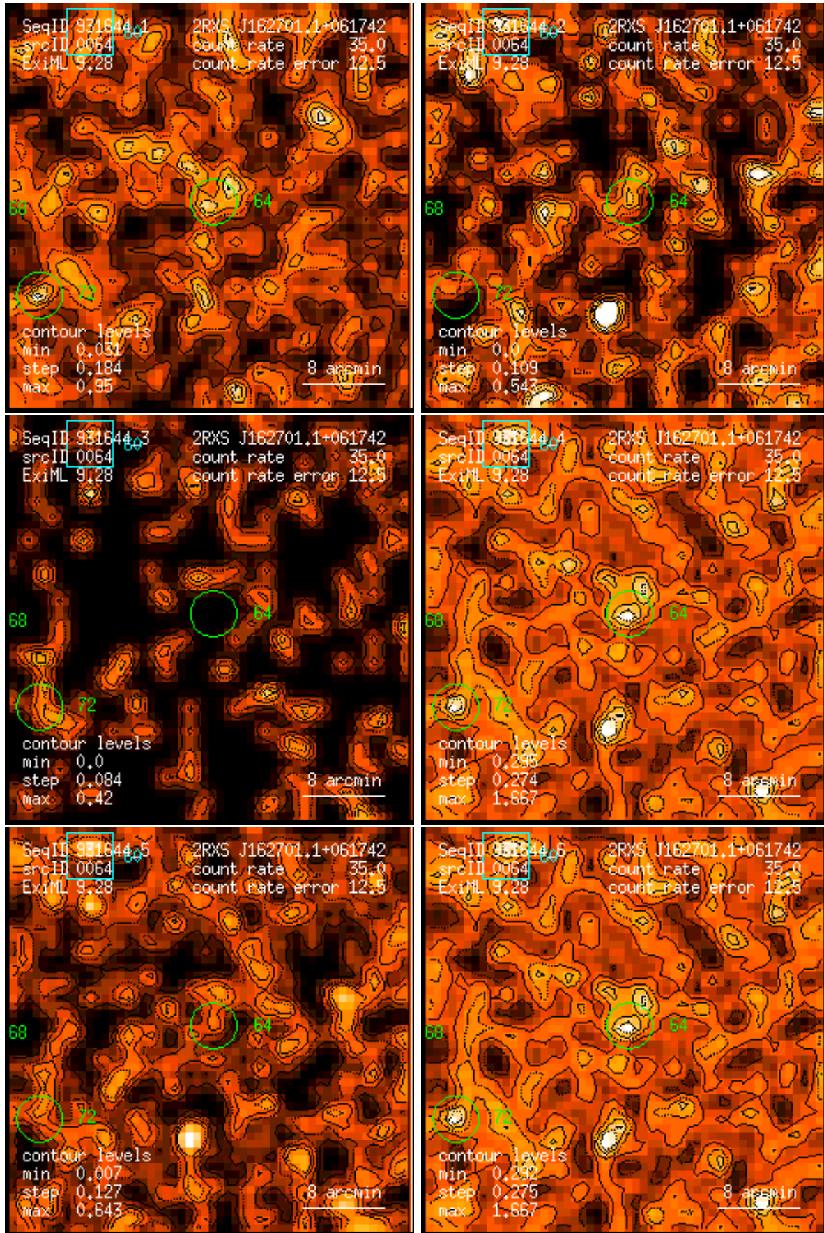
Figure 64: RASS 931644: detection 0064: band rate images, Gaussian filter: (1) PSPC channels 11 – 41, (2) 52 – 90, (3) 91 – 201, (4) 11 – 235, (5) 52 – 201, (6) 11 – 201. Broad band rates in counts/ks. Band rate contour levels in counts/ks/arcmin 2 .
