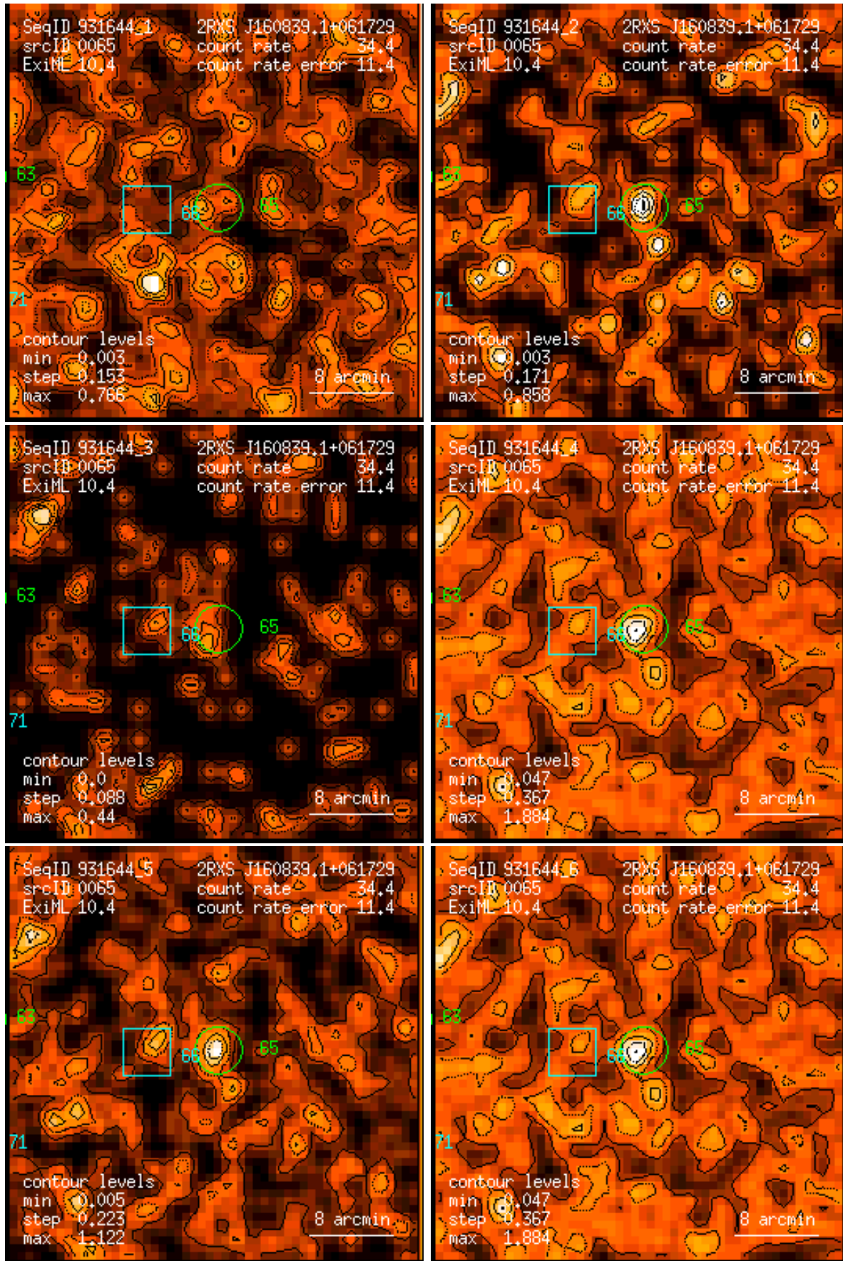
Figure 65: RASS 931644: detection 0065: band rate images, Gaussian filter: (1) PSPC channels 11 – 41, (2) 52 – 90, (3) 91 – 201, (4) 11 – 235, (5) 52 – 201, (6) 11 – 201. Broad band rates in counts/ks. Band rate contour levels in counts/ks/arcmin 2 .
