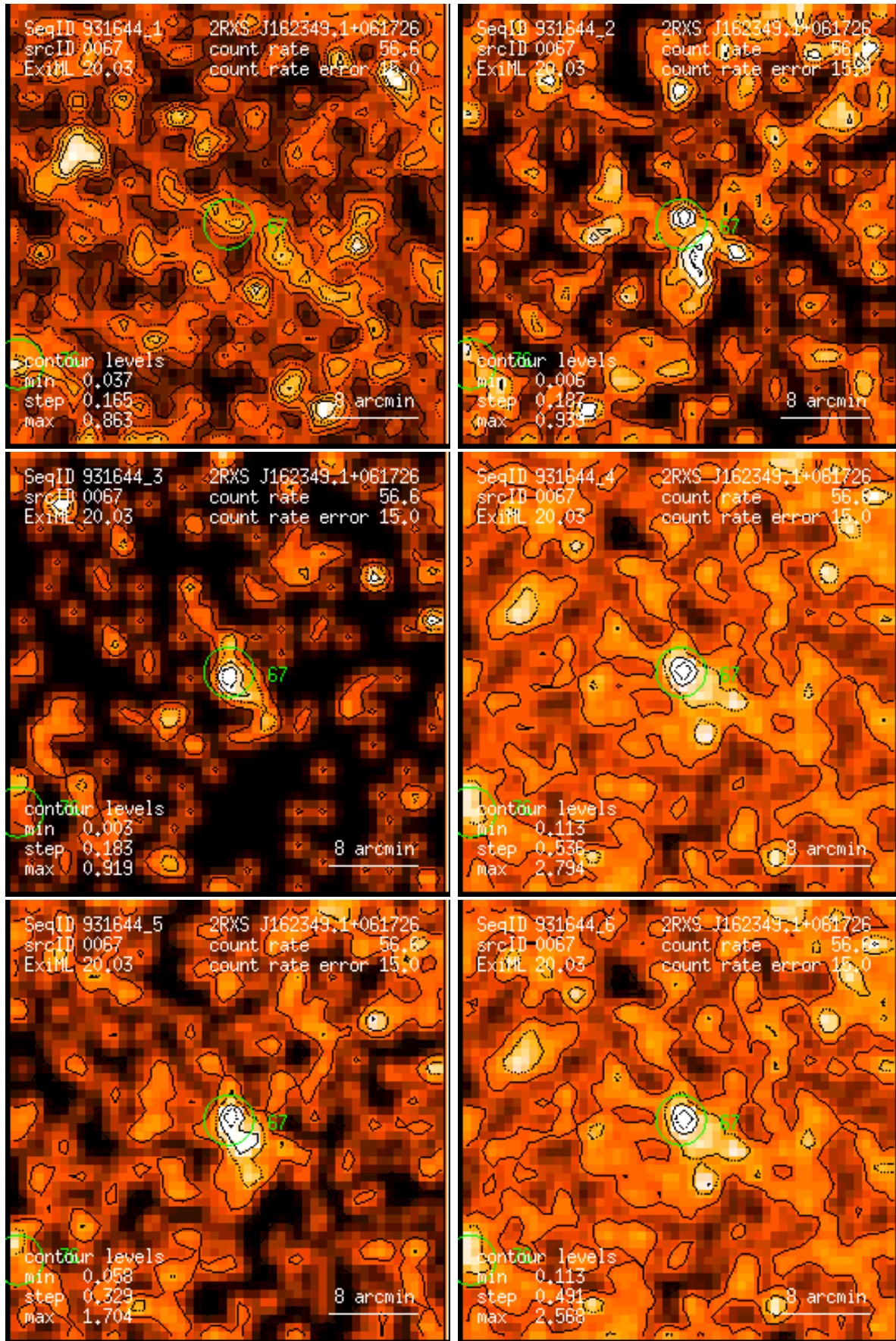
Figure 67: RASS 931644: detection 0067: band rate images, Gaussian filter: (1) PSPC channels 11 – 41, (2) 52 – 90, (3) 91 – 201, (4) 11 – 235, (5) 52 – 201, (6) 11 – 201. Broad band rates in counts/ks. Band rate contour levels in counts/ks/arcmin 2 .
