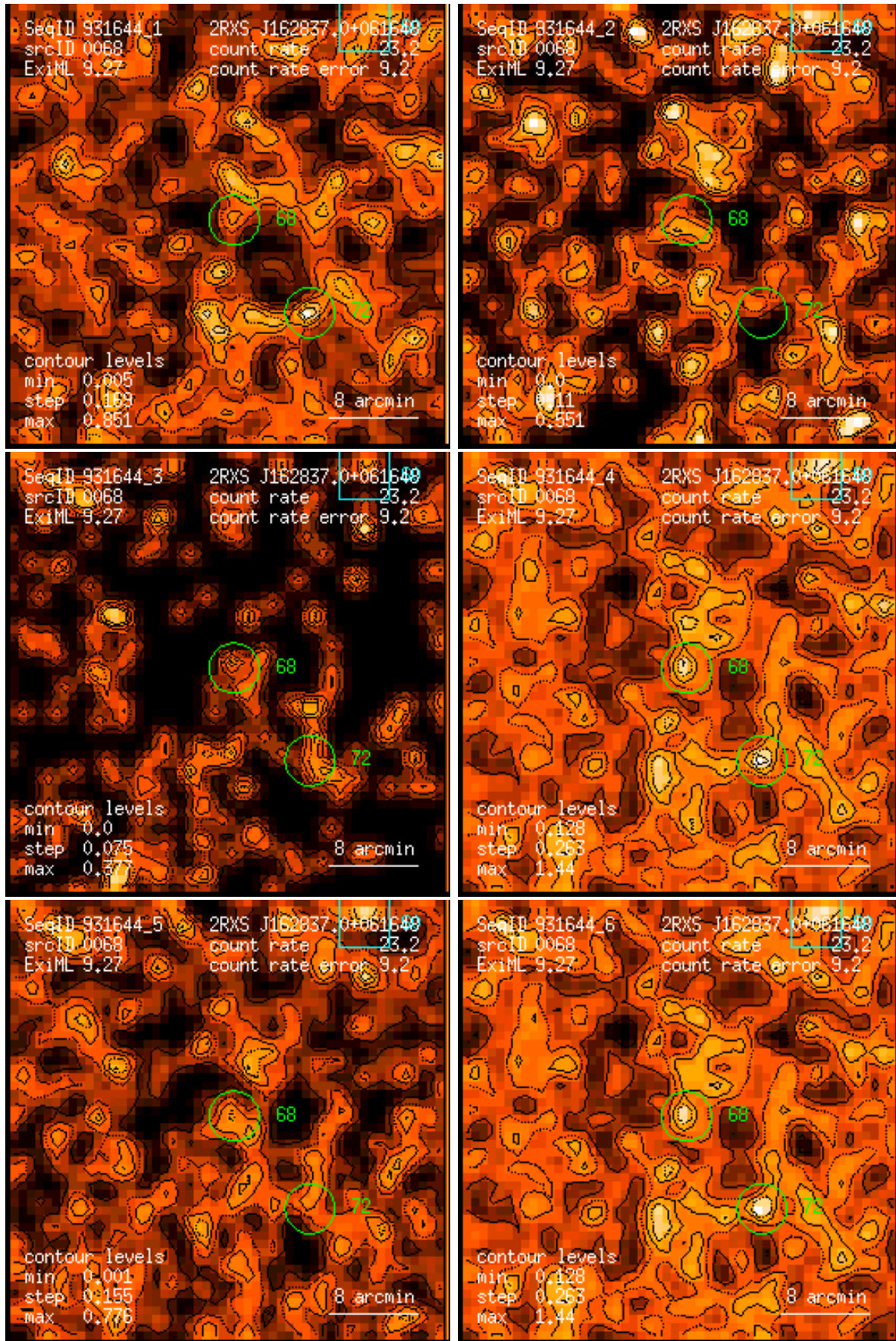
Figure 68: RASS 931644: detection 0068: band rate images, Gaussian filter: (1) PSPC channels 11 – 41, (2) 52 – 90, (3) 91 – 201, (4) 11 – 235, (5) 52 – 201, (6) 11 – 201. Broad band rates in counts/ks. Band rate contour levels in counts/ks/arcmin 2 .
