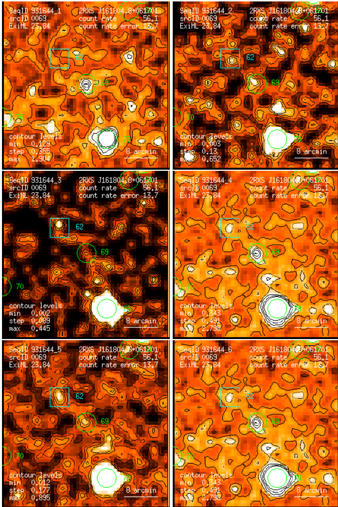
Figure 69: RASS 931644: detection 0069: band rate images, Gaussian filter: (1) PSPC channels 11 – 41, (2) 52 – 90, (3) 91 – 201, (4) 11 – 235, (5) 52 – 201, (6) 11 – 201. Broad band rates in counts/ks. Band rate contour levels in counts/ks/arcmin 2 .
