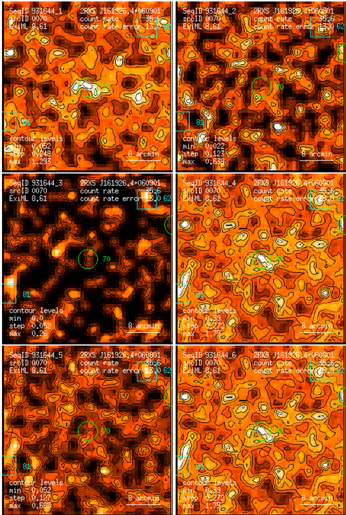
Figure 70: RASS 931644: detection 0070: band rate images, Gaussian filter: (1) PSPC channels 11 – 41, (2) 52 – 90, (3) 91 – 201, (4) 11 – 235, (5) 52 – 201, (6) 11 – 201. Broad band rates in counts/ks. Band rate contour levels in counts/ks/arcmin 2 .
