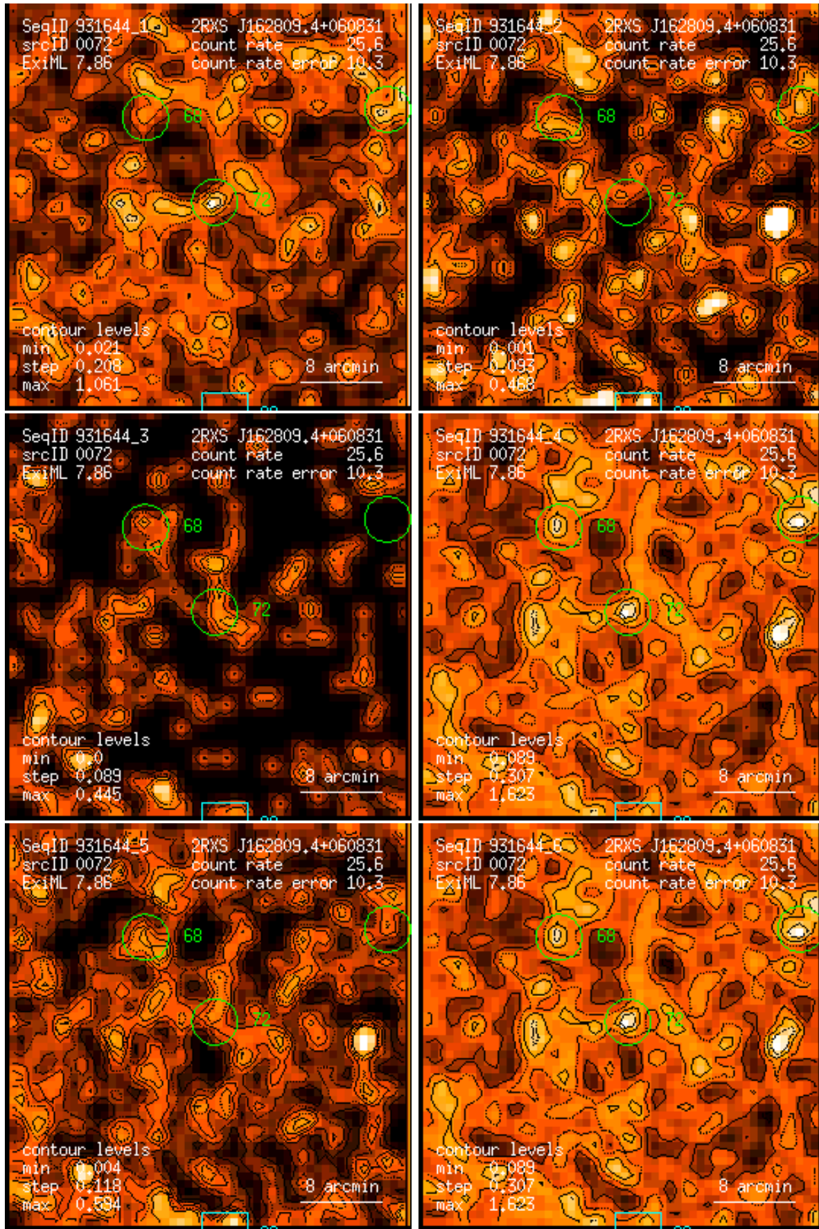
Figure 72: RASS 931644: detection 0072: band rate images, Gaussian filter: (1) PSPC channels 11 – 41, (2) 52 – 90, (3) 91 – 201, (4) 11 – 235, (5) 52 – 201, (6) 11 – 201. Broad band rates in counts/ks. Band rate contour levels in counts/ks/arcmin 2 .
