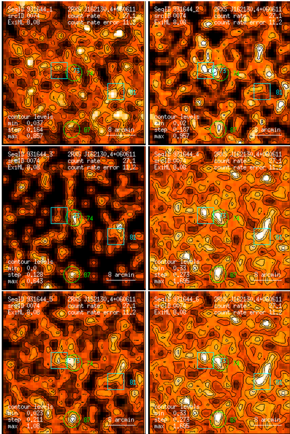
Figure 74: RASS 931644: detection 0074: band rate images, Gaussian filter: (1) PSPC channels 11 – 41, (2) 52 – 90, (3) 91 – 201, (4) 11 – 235, (5) 52 – 201, (6) 11 – 201. Broad band rates in counts/ks. Band rate contour levels in counts/ks/arcmin 2 .
