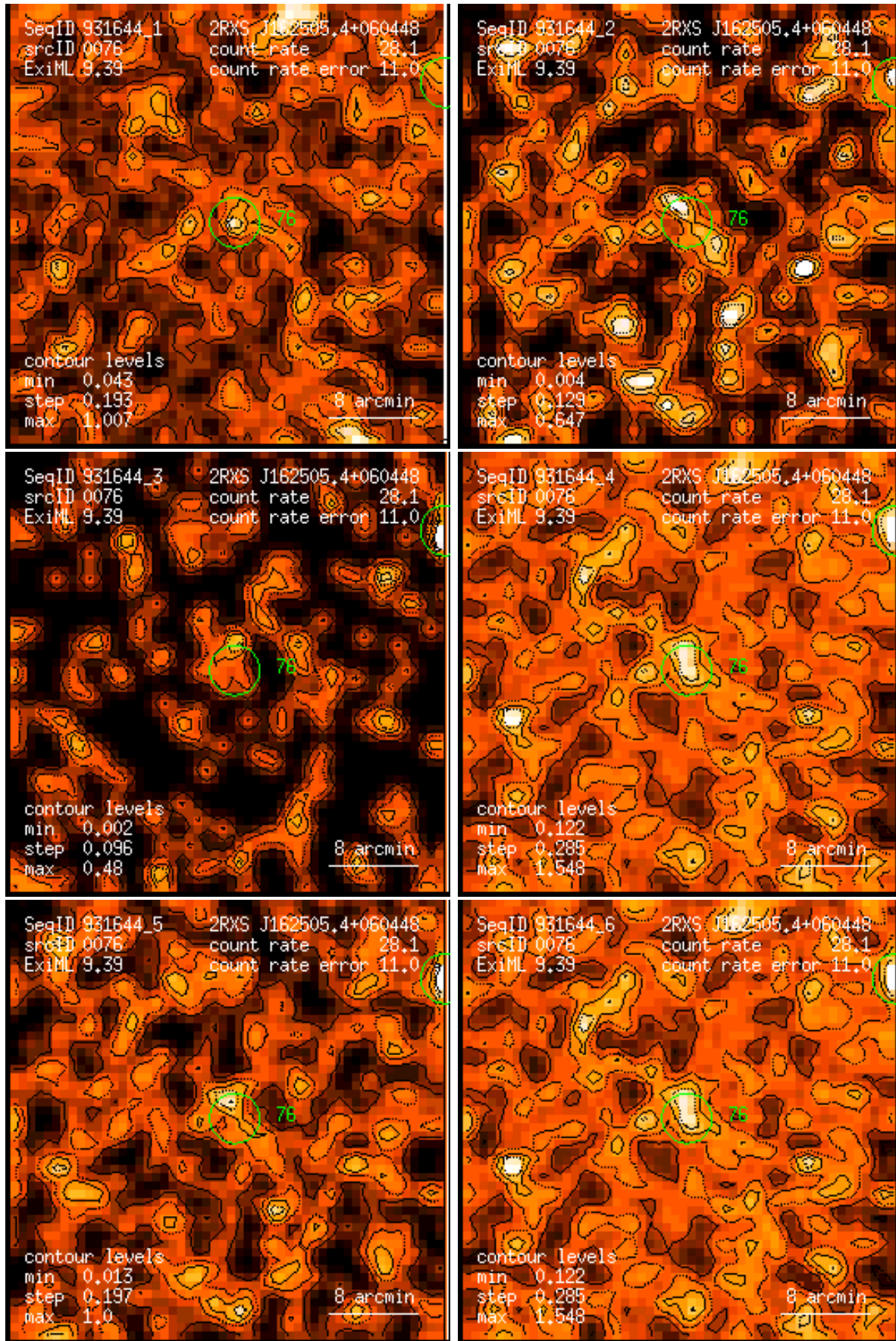
Figure 76: RASS 931644: detection 0076: band rate images, Gaussian filter: (1) PSPC channels 11 – 41, (2) 52 – 90, (3) 91 – 201, (4) 11 – 235, (5) 52 – 201, (6) 11 – 201. Broad band rates in counts/ks. Band rate contour levels in counts/ks/arcmin 2 .
