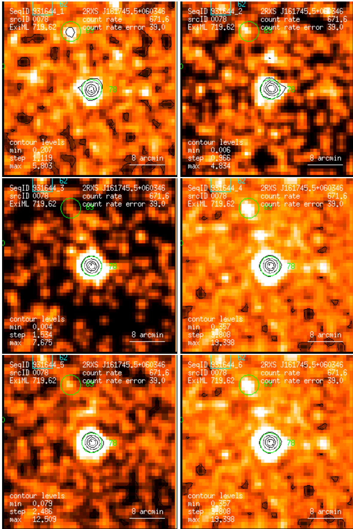
Figure 78: RASS 931644: detection 0078: band rate images, Gaussian filter: (1) PSPC channels 11 – 41, (2) 52 – 90, (3) 91 – 201, (4) 11 – 235, (5) 52 – 201, (6) 11 – 201. Broad band rates in counts/ks. Band rate contour levels in counts/ks/arcmin 2 .
