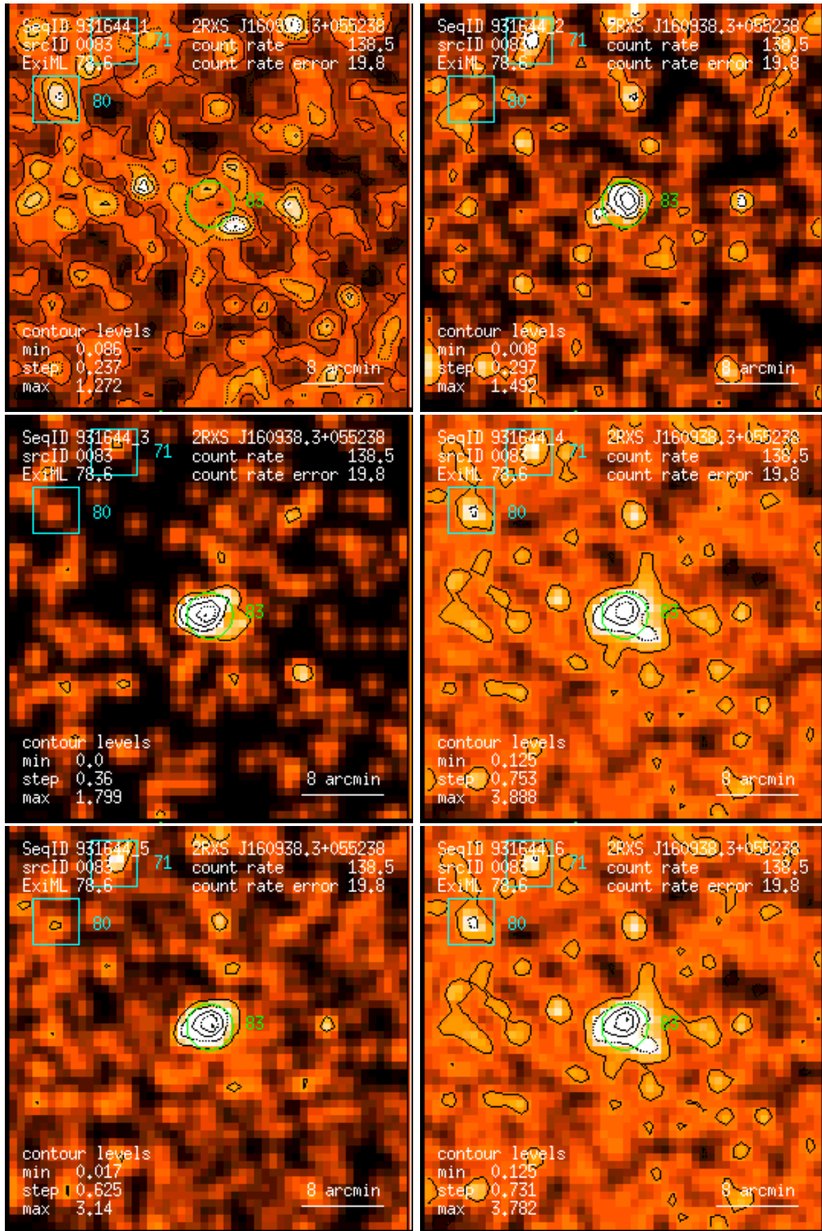
Figure 83: RASS 931644: detection 0083: band rate images, Gaussian filter: (1) PSPC channels 11 – 41, (2) 52 – 90, (3) 91 – 201, (4) 11 – 235, (5) 52 – 201, (6) 11 – 201. Broad band rates in counts/ks. Band rate contour levels in counts/ks/arcmin 2 .
