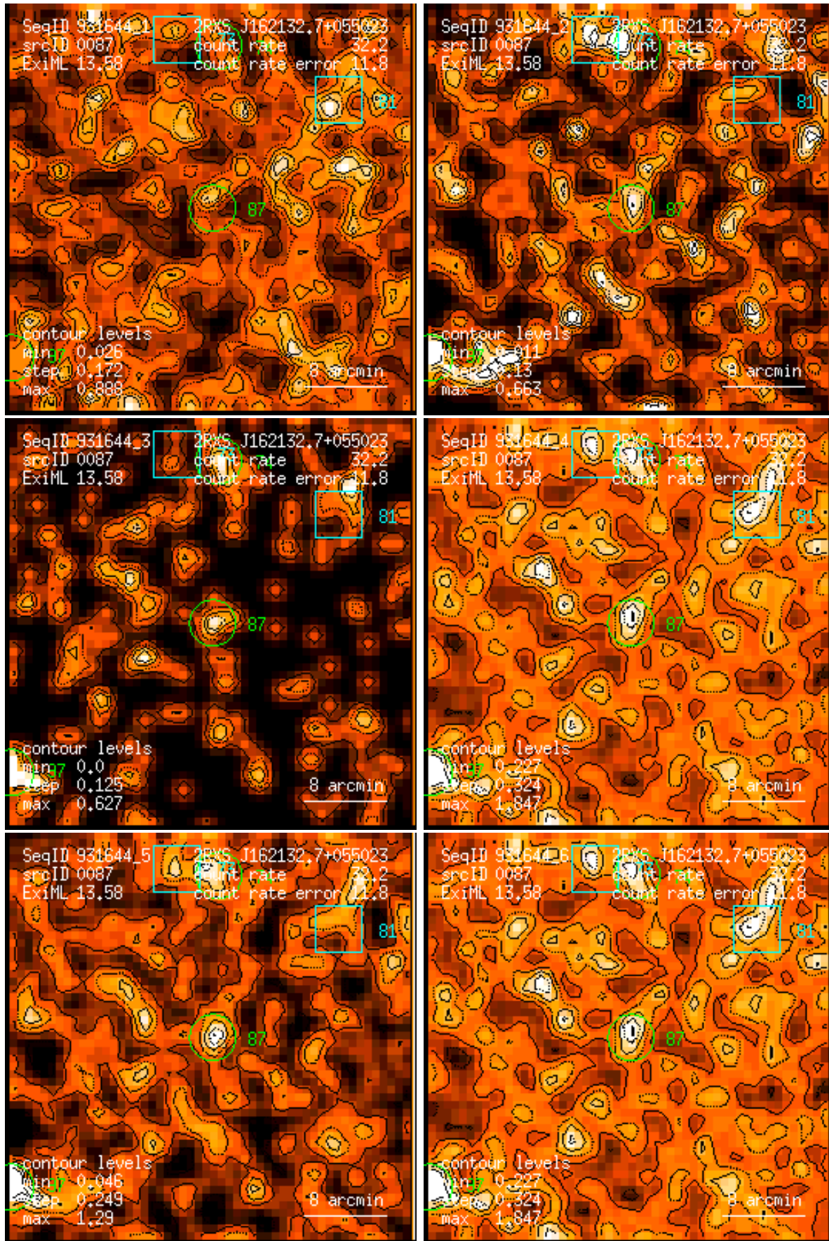
Figure 87: RASS 931644: detection 0087: band rate images, Gaussian filter: (1) PSPC channels 11 – 41, (2) 52 – 90, (3) 91 – 201, (4) 11 – 235, (5) 52 – 201, (6) 11 – 201. Broad band rates in counts/ks. Band rate contour levels in counts/ks/arcmin 2 .
