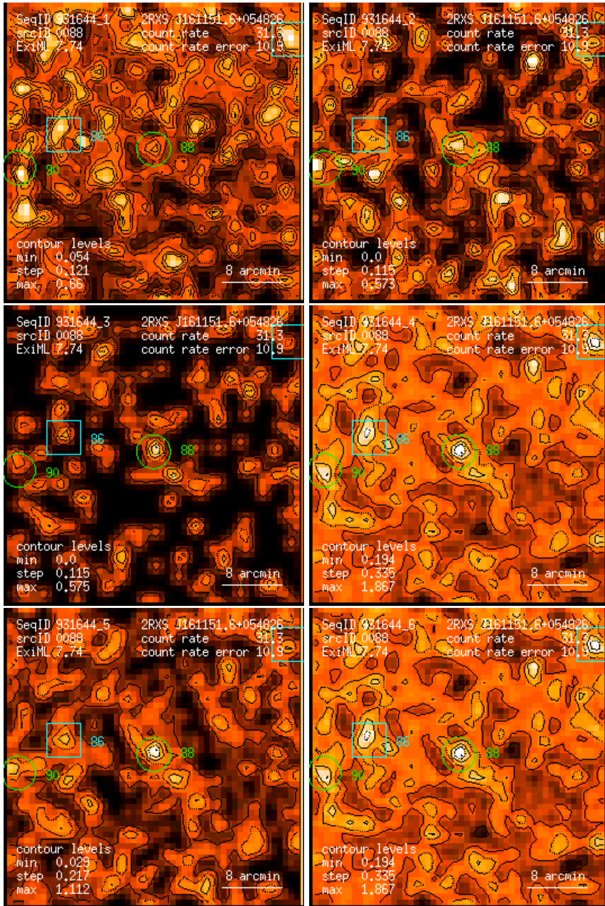
Figure 88: RASS 931644: detection 0088: band rate images, Gaussian filter: (1) PSPC channels 11 – 41, (2) 52 – 90, (3) 91 – 201, (4) 11 – 235, (5) 52 – 201, (6) 11 – 201. Broad band rates in counts/ks. Band rate contour levels in counts/ks/arcmin 2 .
